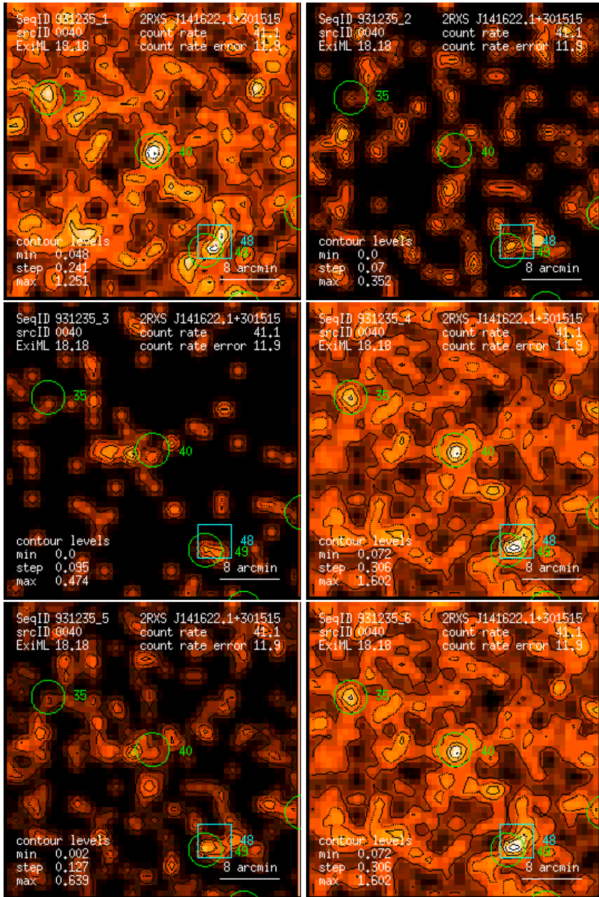
Figure 40: RASS 931235: detection 0040: band rate images, Gaussian filter: (1) PSPC channels 11 – 41, (2) 52 – 90, (3) 91 – 201, (4) 11 – 235, (5) 52 – 201, (6) 11 – 201. Broad band rates in counts/ks. Band rate contour levels in counts/ks/arcmin 2 .
