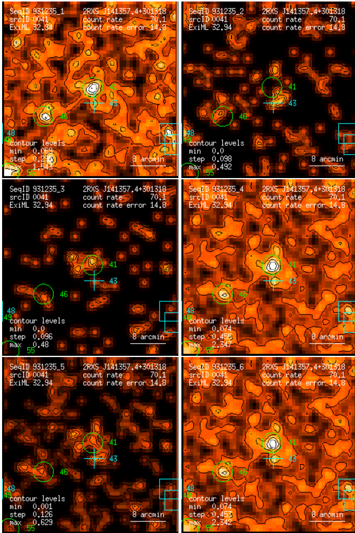
Figure 41: RASS 931235: detection 0041: band rate images, Gaussian filter: (1) PSPC channels 11 – 41, (2) 52 – 90, (3) 91 – 201, (4) 11 – 235, (5) 52 – 201, (6) 11 – 201. Broad band rates in counts/ks. Band rate contour levels in counts/ks/arcmin 2 .
