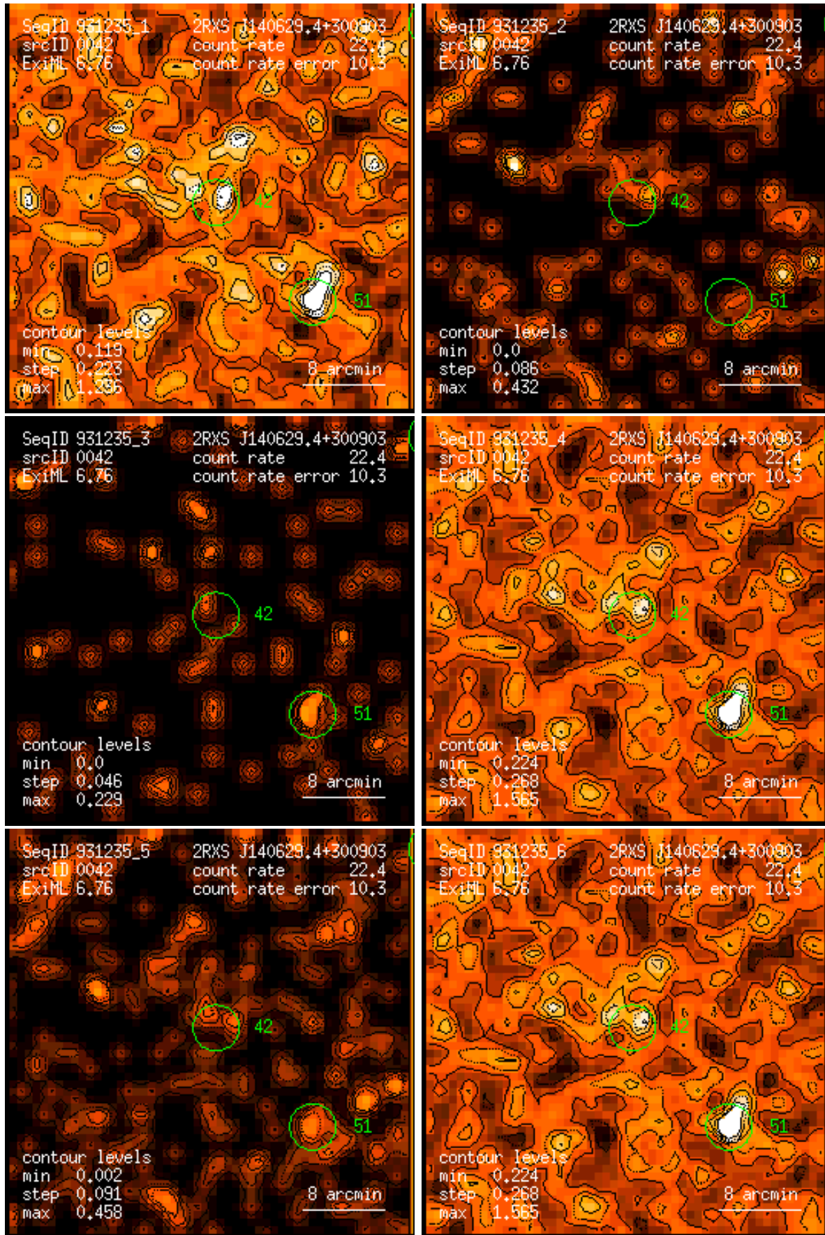
Figure 42: RASS 931235: detection 0042: band rate images, Gaussian filter: (1) PSPC channels 11 – 41, (2) 52 – 90, (3) 91 – 201, (4) 11 – 235, (5) 52 – 201, (6) 11 – 201. Broad band rates in counts/ks. Band rate contour levels in counts/ks/arcmin 2 .
