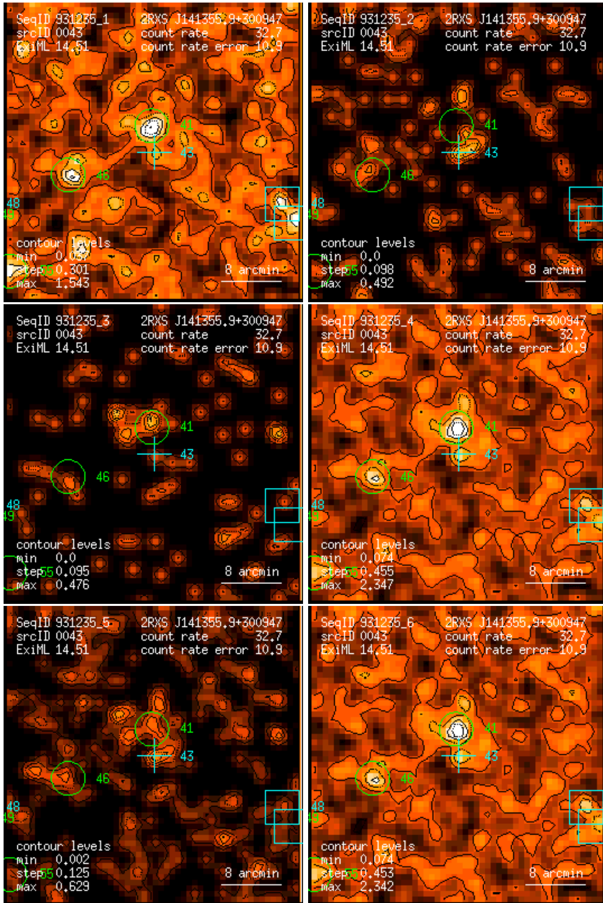
Figure 43: RASS 931235: detection 0043: band rate images, Gaussian filter: (1) PSPC channels 11 – 41, (2) 52 – 90, (3) 91 – 201, (4) 11 – 235, (5) 52 – 201, (6) 11 – 201. Broad band rates in counts/ks. Band rate contour levels in counts/ks/arcmin 2 .
