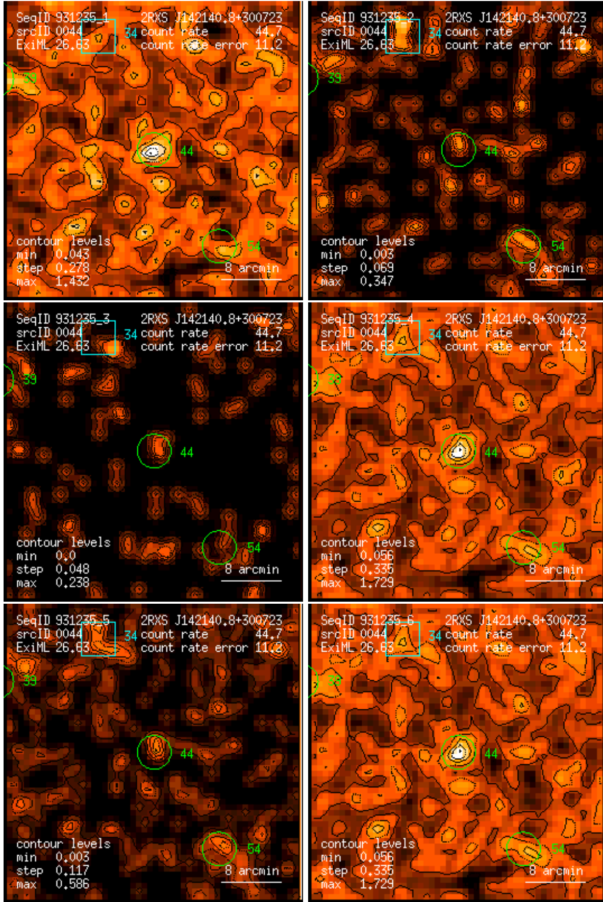
Figure 44: RASS 931235: detection 0044: band rate images, Gaussian filter: (1) PSPC channels 11 – 41, (2) 52 – 90, (3) 91 – 201, (4) 11 – 235, (5) 52 – 201, (6) 11 – 201. Broad band rates in counts/ks. Band rate contour levels in counts/ks/arcmin 2 .
