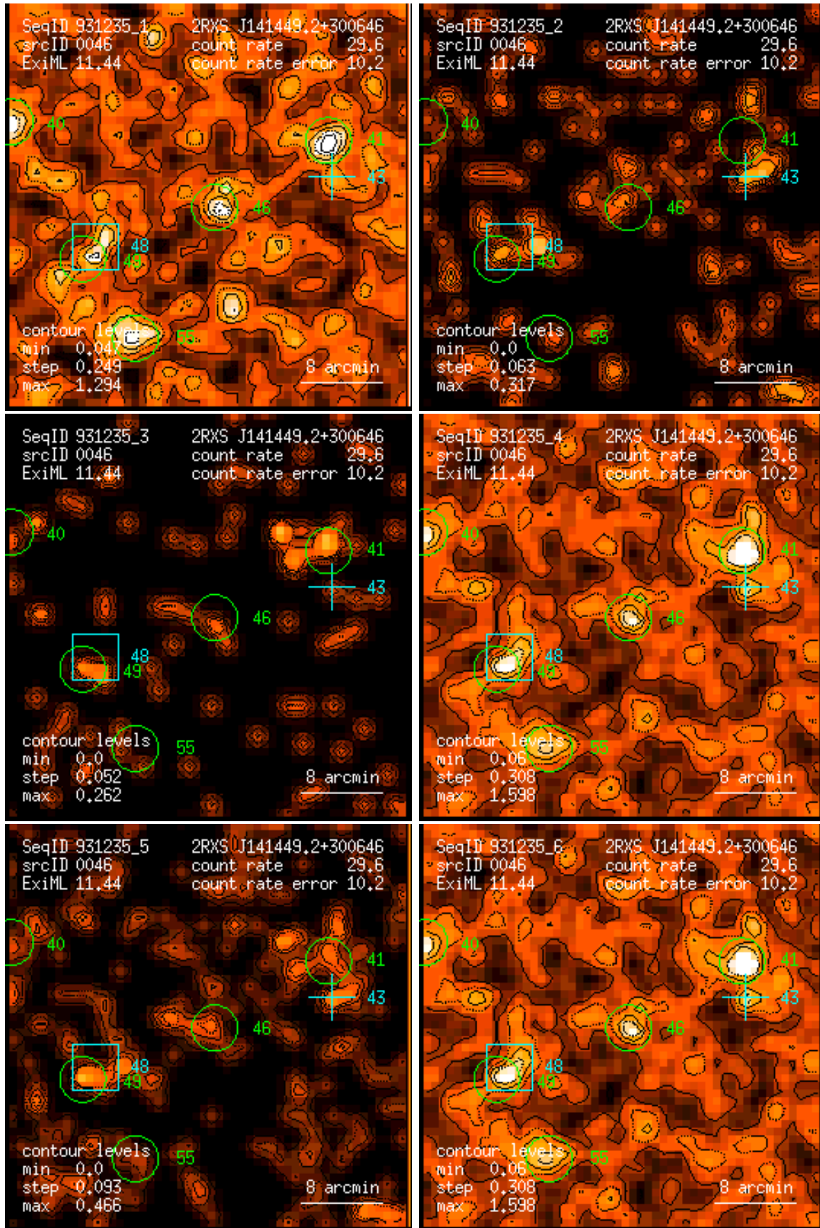
Figure 46: RASS 931235: detection 0046: band rate images, Gaussian filter: (1) PSPC channels 11 – 41, (2) 52 – 90, (3) 91 – 201, (4) 11 – 235, (5) 52 – 201, (6) 11 – 201. Broad band rates in counts/ks. Band rate contour levels in counts/ks/arcmin 2 .
