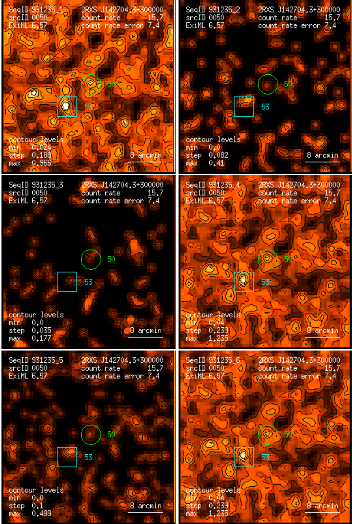
Figure 50: RASS 931235: detection 0050: band rate images, Gaussian filter: (1) PSPC channels 11 – 41, (2) 52 – 90, (3) 91 – 201, (4) 11 – 235, (5) 52 – 201, (6) 11 – 201. Broad band rates in counts/ks. Band rate contour levels in counts/ks/arcmin 2 .
