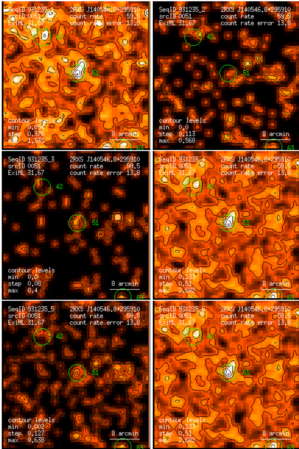
Figure 51: RASS 931235: detection 0051: band rate images, Gaussian filter: (1) PSPC channels 11 – 41, (2) 52 – 90, (3) 91 – 201, (4) 11 – 235, (5) 52 – 201, (6) 11 – 201. Broad band rates in counts/ks. Band rate contour levels in counts/ks/arcmin 2 .
