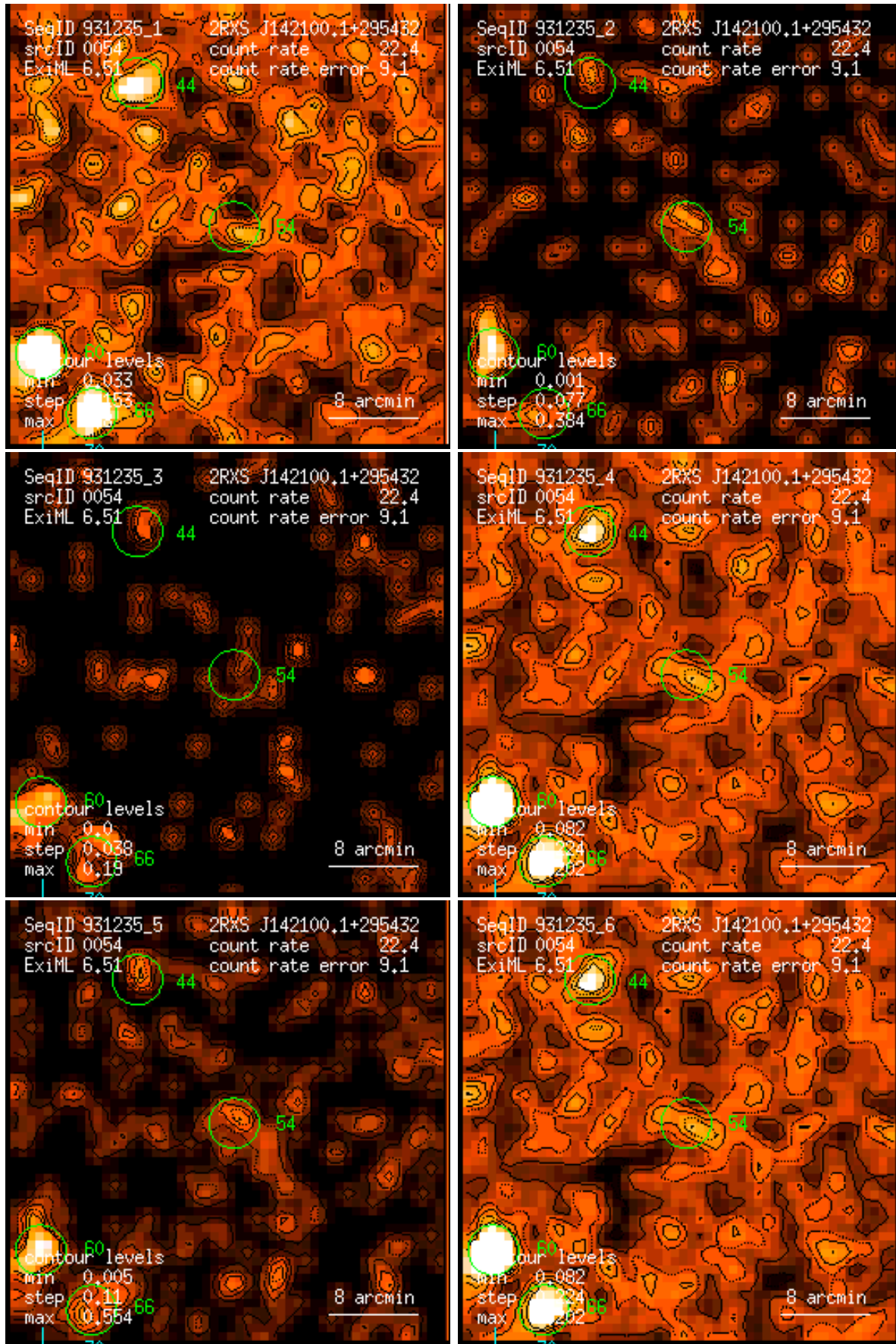
Figure 54: RASS 931235: detection 0054: band rate images, Gaussian filter: (1) PSPC channels 11 – 41, (2) 52 – 90, (3) 91 – 201, (4) 11 – 235, (5) 52 – 201, (6) 11 – 201. Broad band rates in counts/ks. Band rate contour levels in counts/ks/arcmin 2 .
