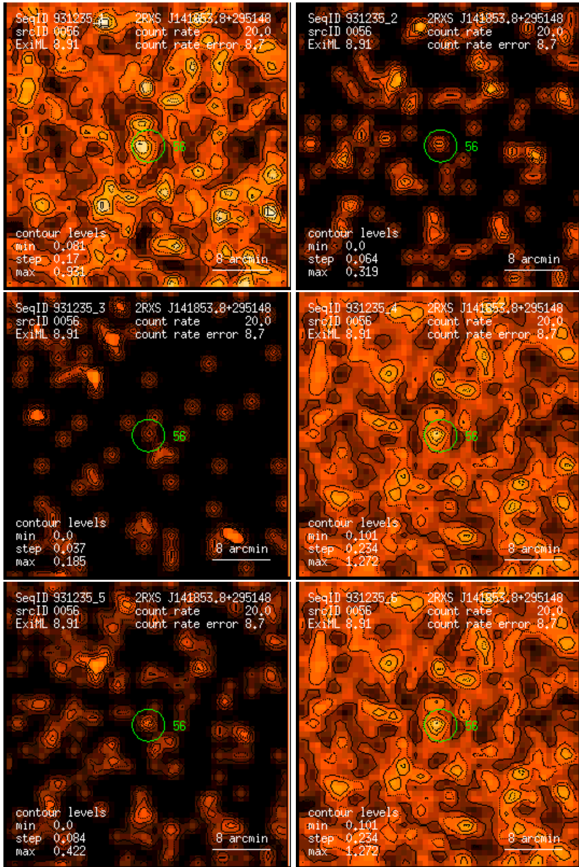
Figure 56: RASS 931235: detection 0056: band rate images, Gaussian filter: (1) PSPC channels 11 – 41, (2) 52 – 90, (3) 91 – 201, (4) 11 – 235, (5) 52 – 201, (6) 11 – 201. Broad band rates in counts/ks. Band rate contour levels in counts/ks/arcmin 2 .
