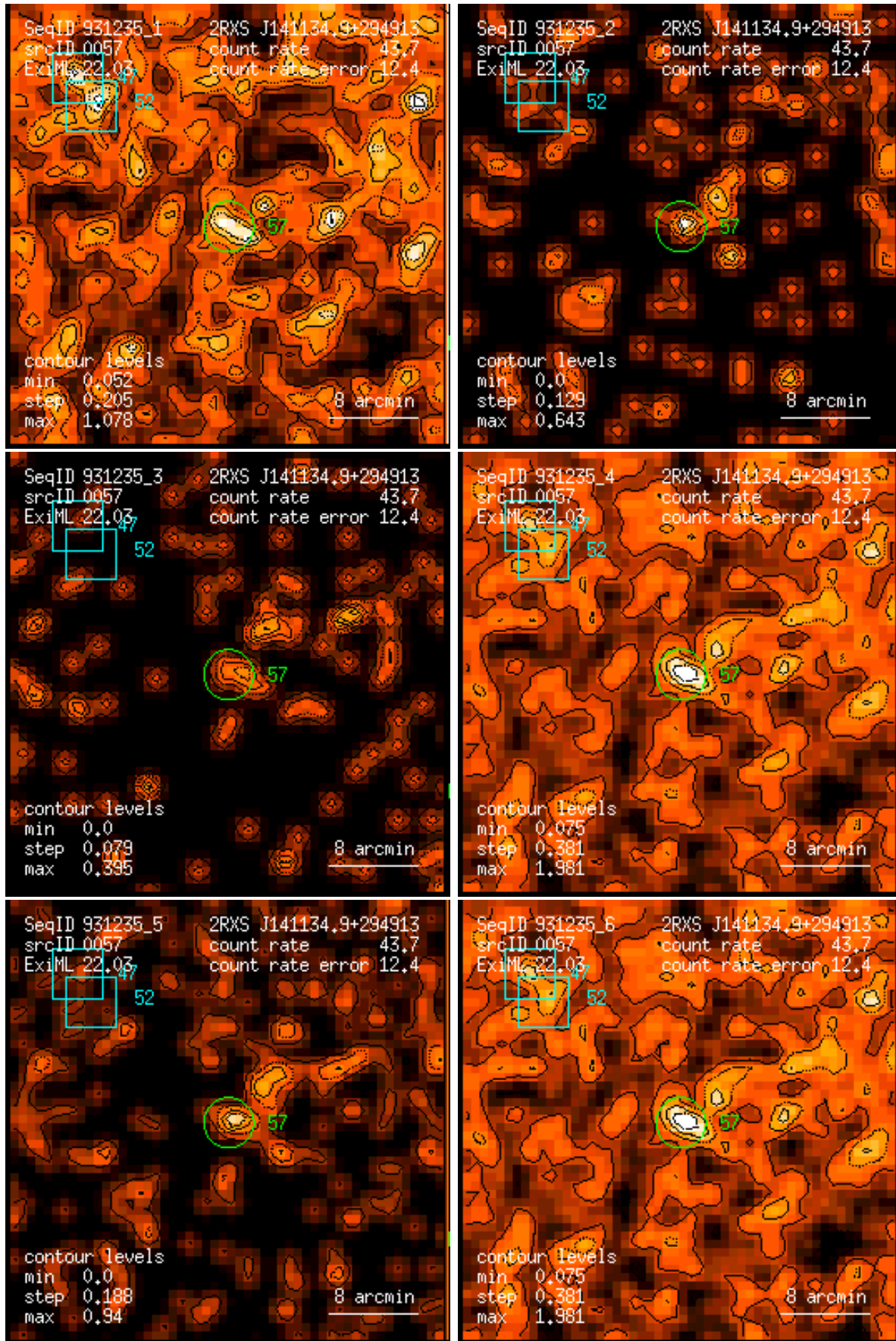
Figure 57: RASS 931235: detection 0057: band rate images, Gaussian filter: (1) PSPC channels 11 – 41, (2) 52 – 90, (3) 91 – 201, (4) 11 – 235, (5) 52 – 201, (6) 11 – 201. Broad band rates in counts/ks. Band rate contour levels in counts/ks/arcmin 2 .
