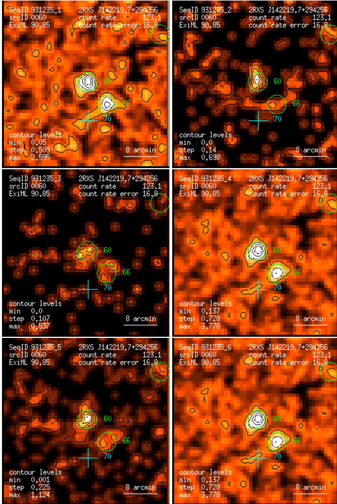
Figure 60: RASS 931235: detection 0060: band rate images, Gaussian filter: (1) PSPC channels 11 – 41, (2) 52 – 90, (3) 91 – 201, (4) 11 – 235, (5) 52 – 201, (6) 11 – 201. Broad band rates in counts/ks. Band rate contour levels in counts/ks/arcmin 2 .
