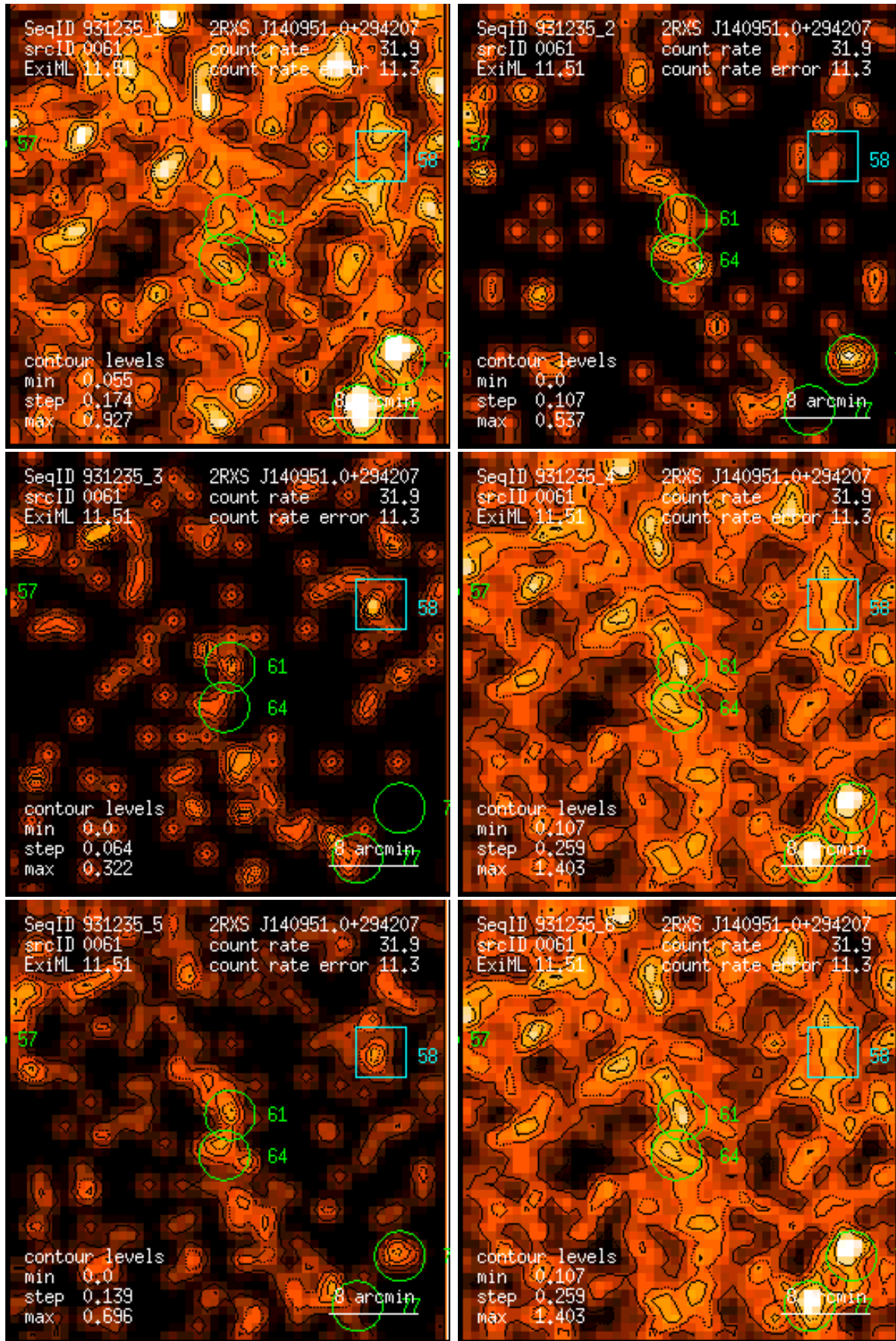
Figure 61: RASS 931235: detection 0061: band rate images, Gaussian filter: (1) PSPC channels 11 – 41, (2) 52 – 90, (3) 91 – 201, (4) 11 – 235, (5) 52 – 201, (6) 11 – 201. Broad band rates in counts/ks. Band rate contour levels in counts/ks/arcmin 2 .
