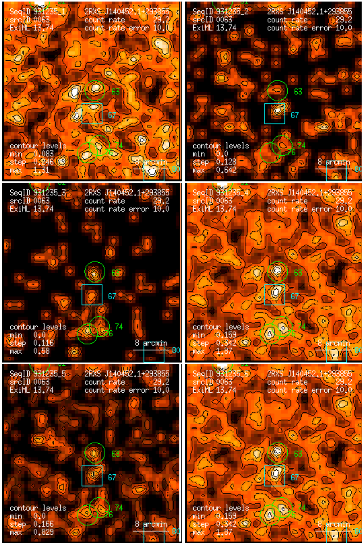
Figure 63: RASS 931235: detection 0063: band rate images, Gaussian filter: (1) PSPC channels 11 – 41, (2) 52 – 90, (3) 91 – 201, (4) 11 – 235, (5) 52 – 201, (6) 11 – 201. Broad band rates in counts/ks. Band rate contour levels in counts/ks/arcmin 2 .
