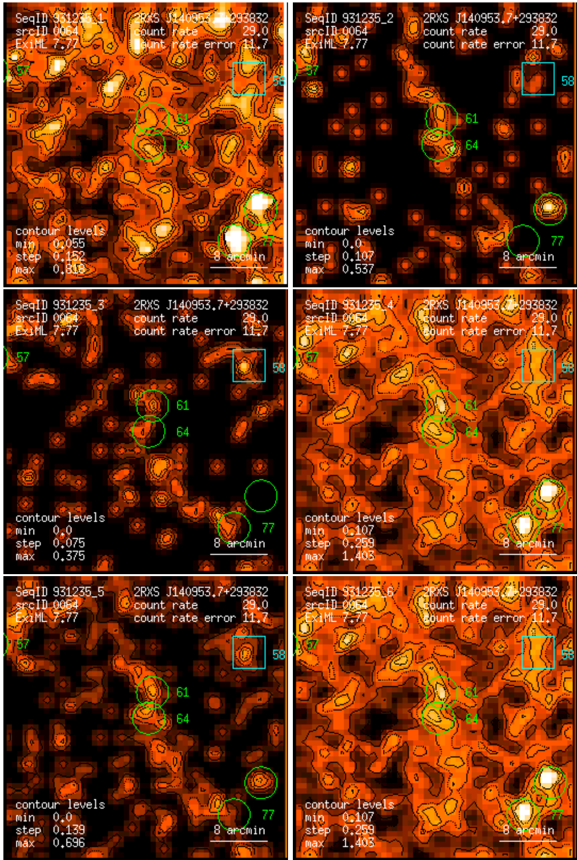
Figure 64: RASS 931235: detection 0064: band rate images, Gaussian filter: (1) PSPC channels 11 – 41, (2) 52 – 90, (3) 91 – 201, (4) 11 – 235, (5) 52 – 201, (6) 11 – 201. Broad band rates in counts/ks. Band rate contour levels in counts/ks/arcmin 2 .
