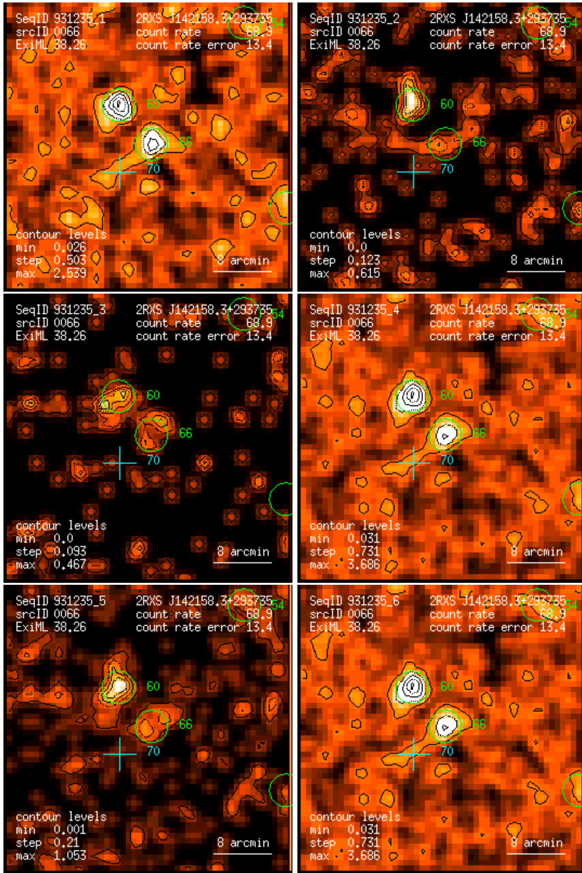
Figure 66: RASS 931235: detection 0066: band rate images, Gaussian filter: (1) PSPC channels 11 – 41, (2) 52 – 90, (3) 91 – 201, (4) 11 – 235, (5) 52 – 201, (6) 11 – 201. Broad band rates in counts/ks. Band rate contour levels in counts/ks/arcmin 2 .
