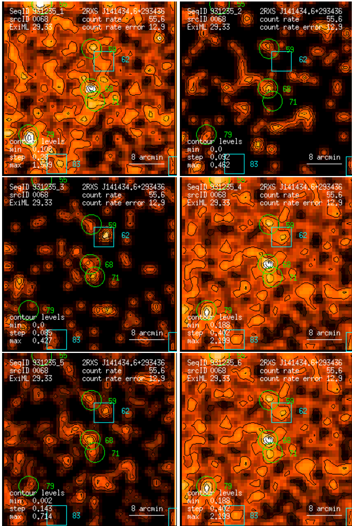
Figure 68: RASS 931235: detection 0068: band rate images, Gaussian filter: (1) PSPC channels 11 – 41, (2) 52 – 90, (3) 91 – 201, (4) 11 – 235, (5) 52 – 201, (6) 11 – 201. Broad band rates in counts/ks. Band rate contour levels in counts/ks/arcmin 2 .
