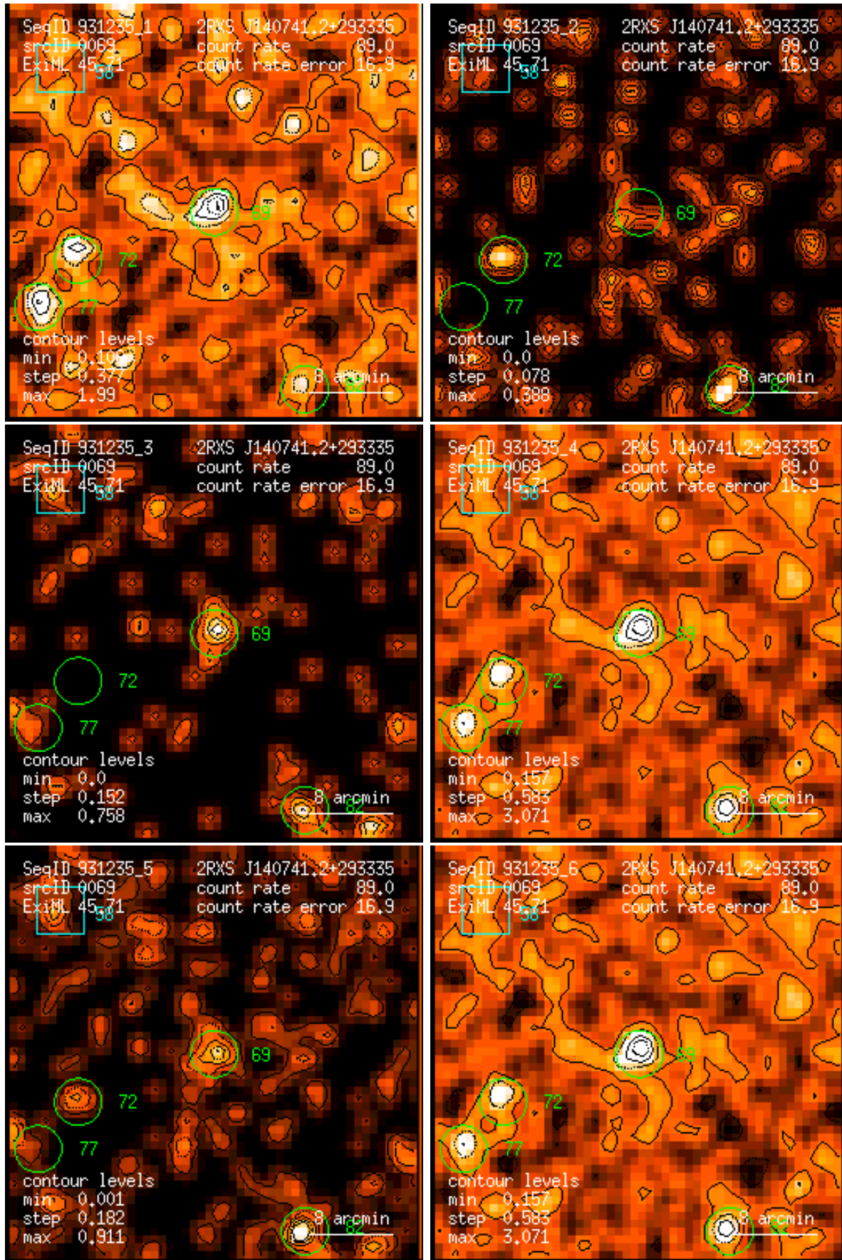
Figure 69: RASS 931235: detection 0069: band rate images, Gaussian filter: (1) PSPC channels 11 – 41, (2) 52 – 90, (3) 91 – 201, (4) 11 – 235, (5) 52 – 201, (6) 11 – 201. Broad band rates in counts/ks. Band rate contour levels in counts/ks/arcmin 2 .
