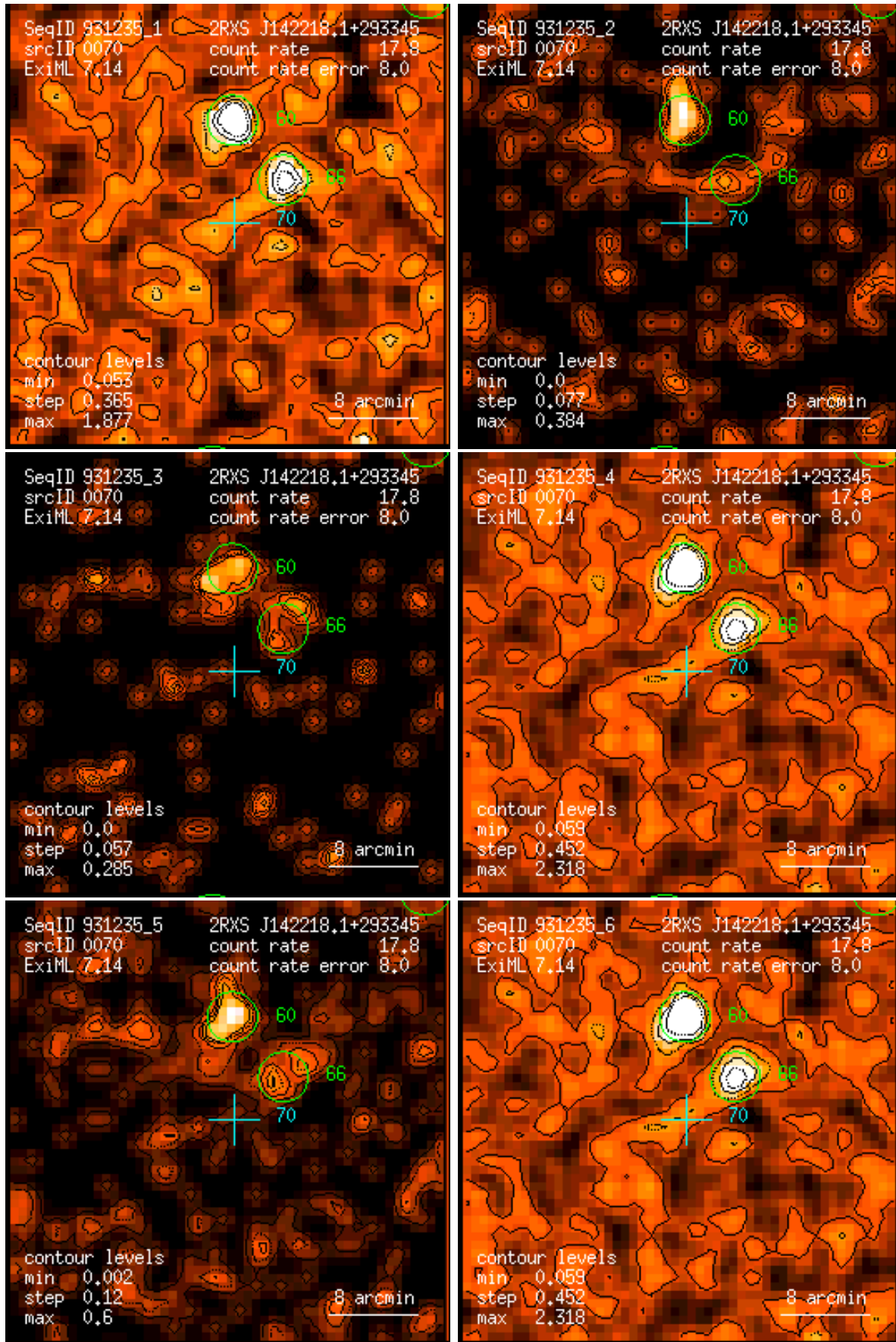
Figure 70: RASS 931235: detection 0070: band rate images, Gaussian filter: (1) PSPC channels 11 – 41, (2) 52 – 90, (3) 91 – 201, (4) 11 – 235, (5) 52 – 201, (6) 11 – 201. Broad band rates in counts/ks. Band rate contour levels in counts/ks/arcmin 2 .
