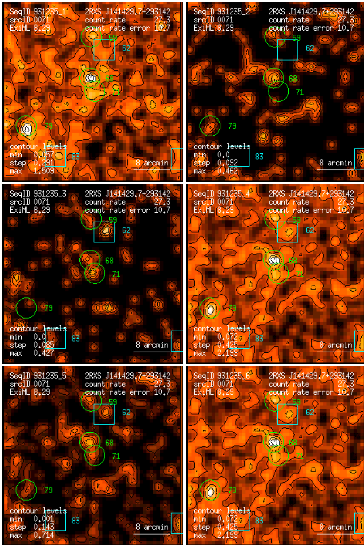
Figure 71: RASS 931235: detection 0071: band rate images, Gaussian filter: (1) PSPC channels 11 – 41, (2) 52 – 90, (3) 91 – 201, (4) 11 – 235, (5) 52 – 201, (6) 11 – 201. Broad band rates in counts/ks. Band rate contour levels in counts/ks/arcmin 2 .
