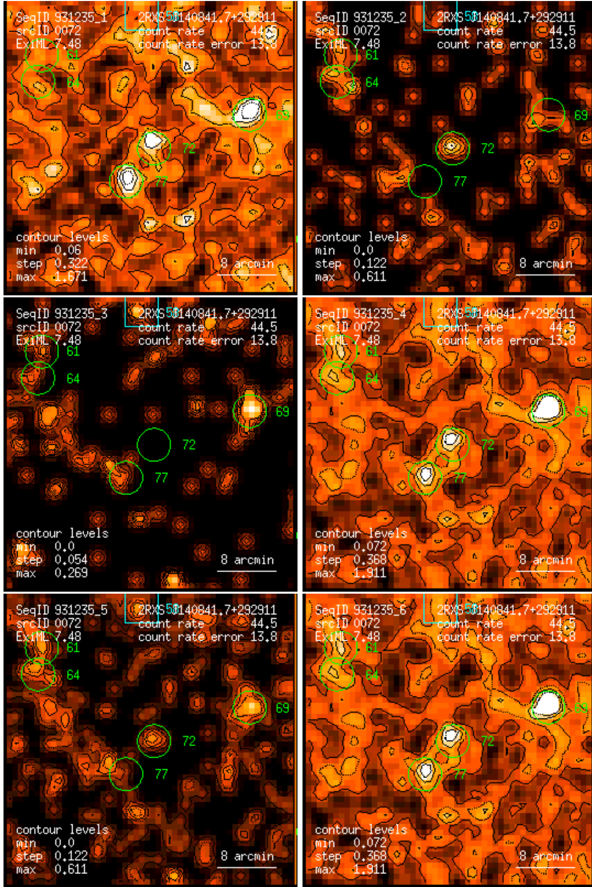
Figure 72: RASS 931235: detection 0072: band rate images, Gaussian filter: (1) PSPC channels 11 – 41, (2) 52 – 90, (3) 91 – 201, (4) 11 – 235, (5) 52 – 201, (6) 11 – 201. Broad band rates in counts/ks. Band rate contour levels in counts/ks/arcmin 2 .
