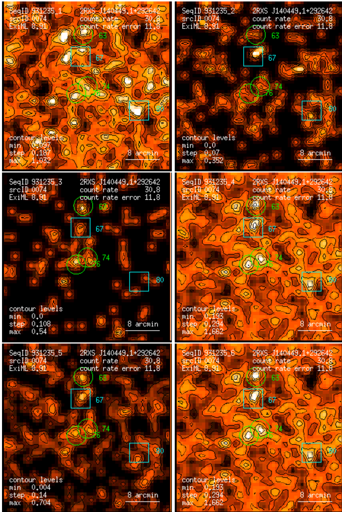
Figure 74: RASS 931235: detection 0074: band rate images, Gaussian filter: (1) PSPC channels 11 – 41, (2) 52 – 90, (3) 91 – 201, (4) 11 – 235, (5) 52 – 201, (6) 11 – 201. Broad band rates in counts/ks. Band rate contour levels in counts/ks/arcmin 2 .
