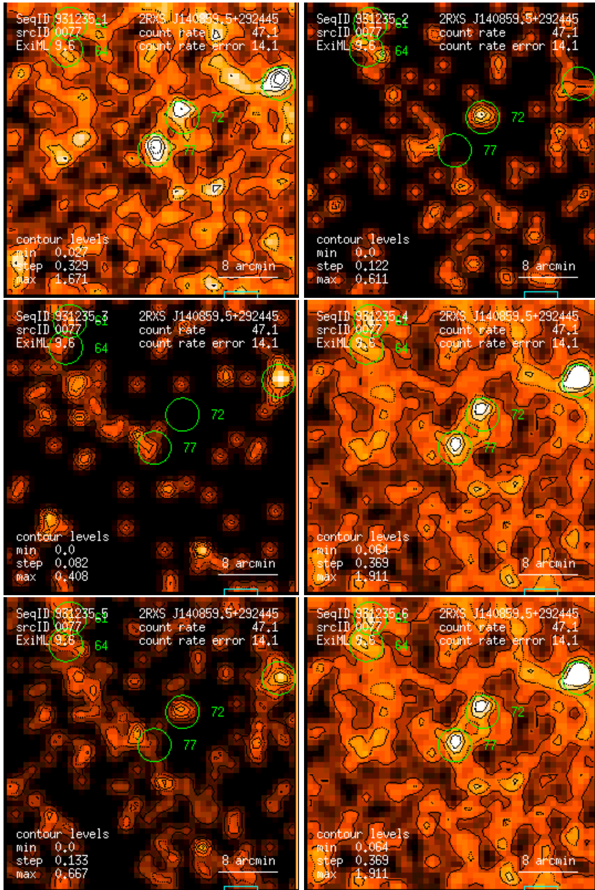
Figure 77: RASS 931235: detection 0077: band rate images, Gaussian filter: (1) PSPC channels 11 – 41, (2) 52 – 90, (3) 91 – 201, (4) 11 – 235, (5) 52 – 201, (6) 11 – 201. Broad band rates in counts/ks. Band rate contour levels in counts/ks/arcmin 2 .
