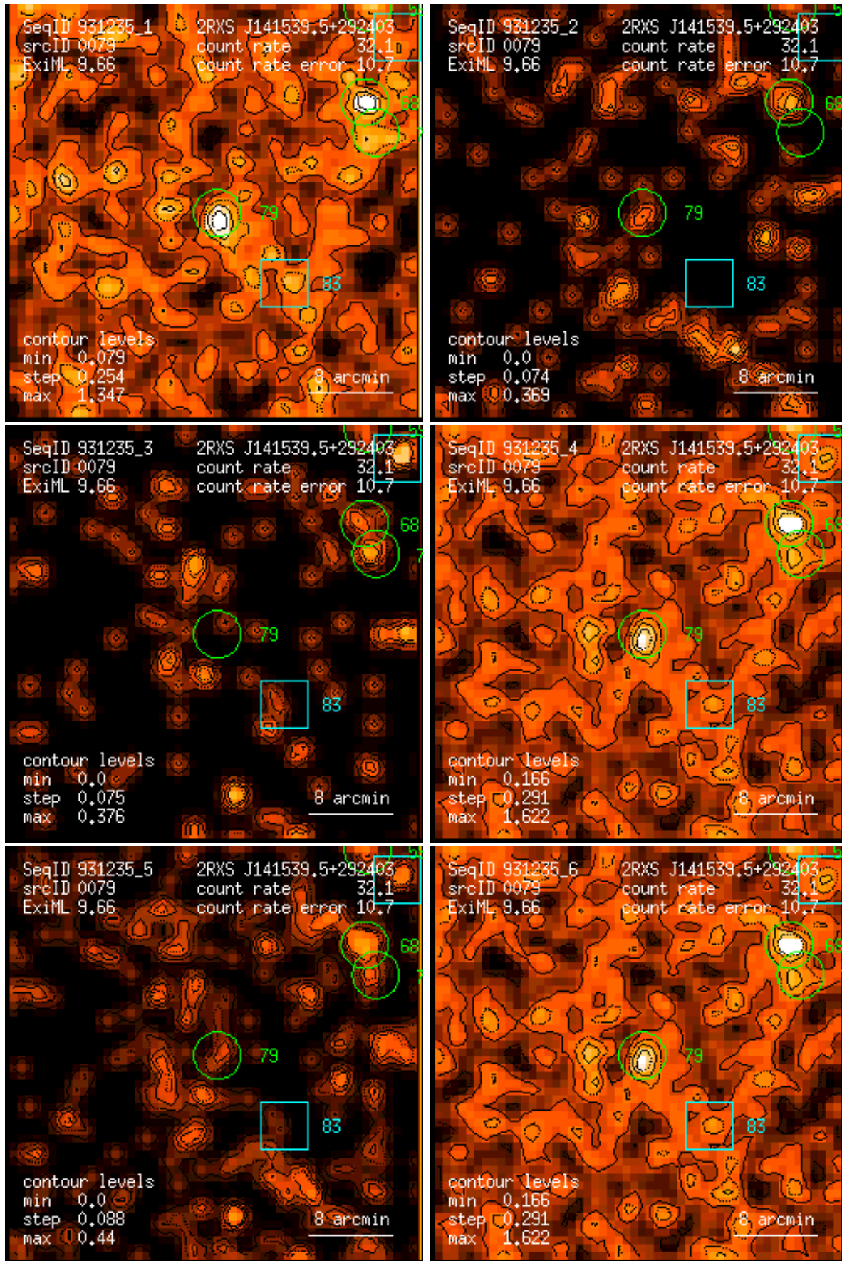
Figure 79: RASS 931235: detection 0079: band rate images, Gaussian filter: (1) PSPC channels 11 – 41, (2) 52 – 90, (3) 91 – 201, (4) 11 – 235, (5) 52 – 201, (6) 11 – 201. Broad band rates in counts/ks. Band rate contour levels in counts/ks/arcmin 2 .
