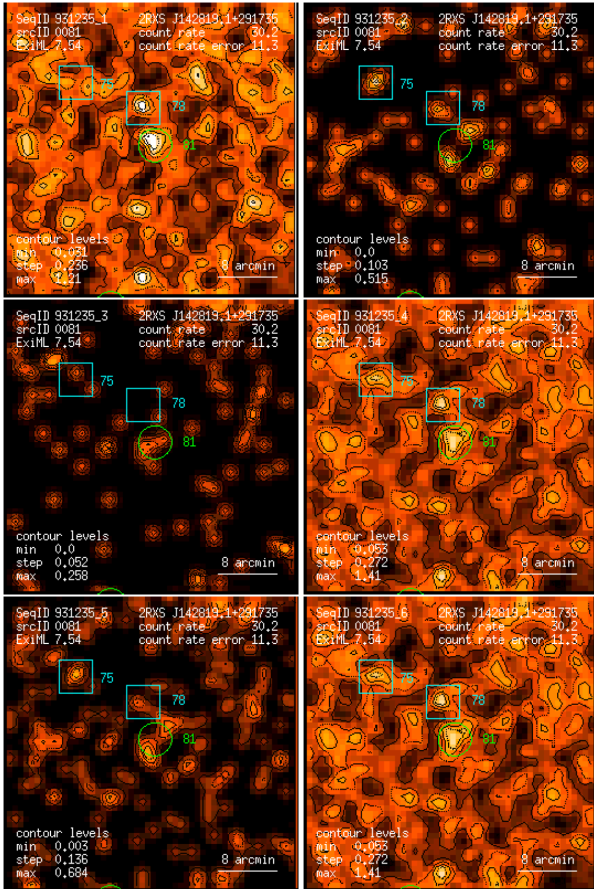
Figure 81: RASS 931235: detection 0081: band rate images, Gaussian filter: (1) PSPC channels 11 – 41, (2) 52 – 90, (3) 91 – 201, (4) 11 – 235, (5) 52 – 201, (6) 11 – 201. Broad band rates in counts/ks. Band rate contour levels in counts/ks/arcmin 2 .
