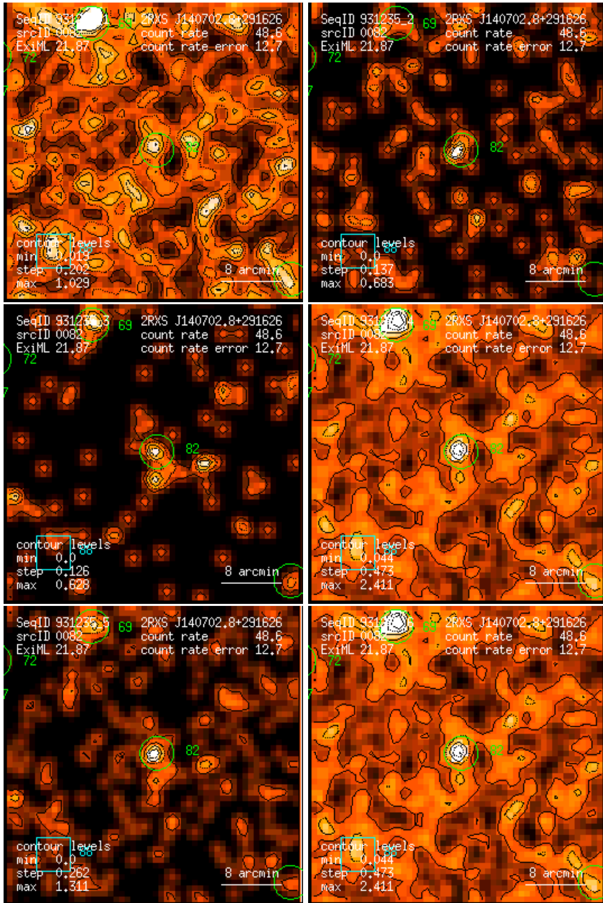
Figure 82: RASS 931235: detection 0082: band rate images, Gaussian filter: (1) PSPC channels 11 – 41, (2) 52 – 90, (3) 91 – 201, (4) 11 – 235, (5) 52 – 201, (6) 11 – 201. Broad band rates in counts/ks. Band rate contour levels in counts/ks/arcmin 2 .
