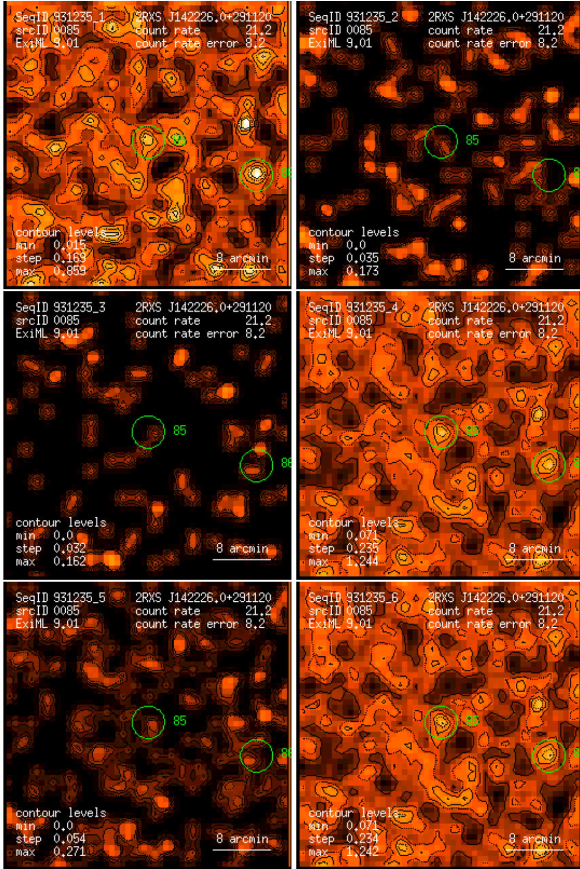
Figure 85: RASS 931235: detection 0085: band rate images, Gaussian filter: (1) PSPC channels 11 – 41, (2) 52 – 90, (3) 91 – 201, (4) 11 – 235, (5) 52 – 201, (6) 11 – 201. Broad band rates in counts/ks. Band rate contour levels in counts/ks/arcmin 2 .
