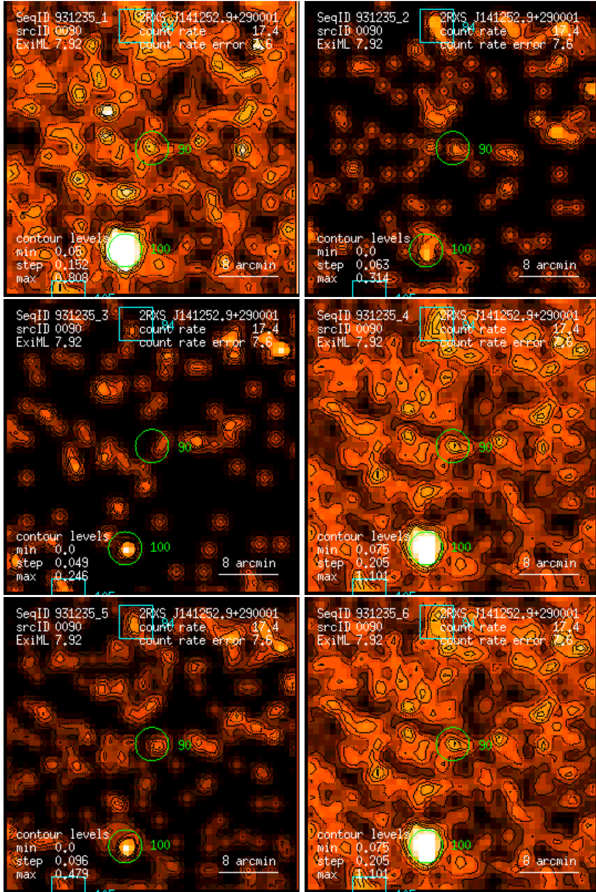
Figure 90: RASS 931235: detection 0090: band rate images, Gaussian filter: (1) PSPC channels 11 – 41, (2) 52 – 90, (3) 91 – 201, (4) 11 – 235, (5) 52 – 201, (6) 11 – 201. Broad band rates in counts/ks. Band rate contour levels in counts/ks/arcmin 2 .
