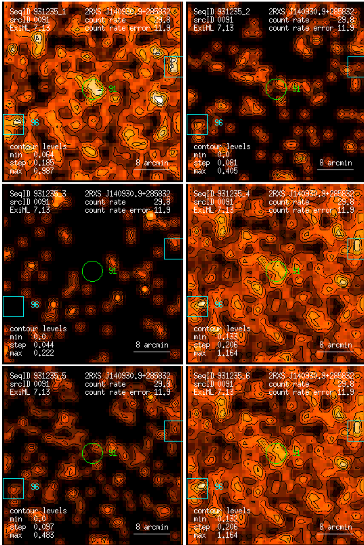
Figure 91: RASS 931235: detection 0091: band rate images, Gaussian filter: (1) PSPC channels 11 – 41, (2) 52 – 90, (3) 91 – 201, (4) 11 – 235, (5) 52 – 201, (6) 11 – 201. Broad band rates in counts/ks. Band rate contour levels in counts/ks/arcmin 2 .
