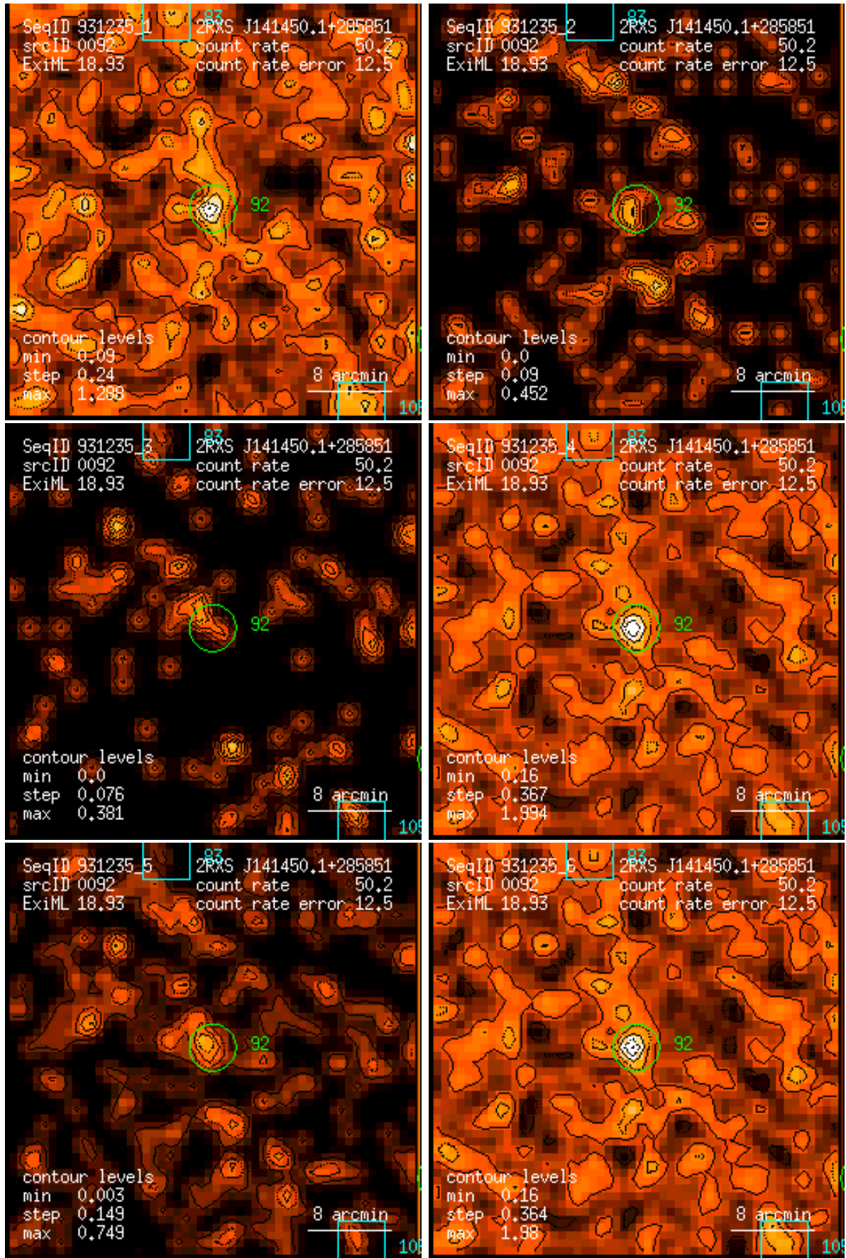
Figure 92: RASS 931235: detection 0092: band rate images, Gaussian filter: (1) PSPC channels 11 – 41, (2) 52 – 90, (3) 91 – 201, (4) 11 – 235, (5) 52 – 201, (6) 11 – 201. Broad band rates in counts/ks. Band rate contour levels in counts/ks/arcmin 2 .
