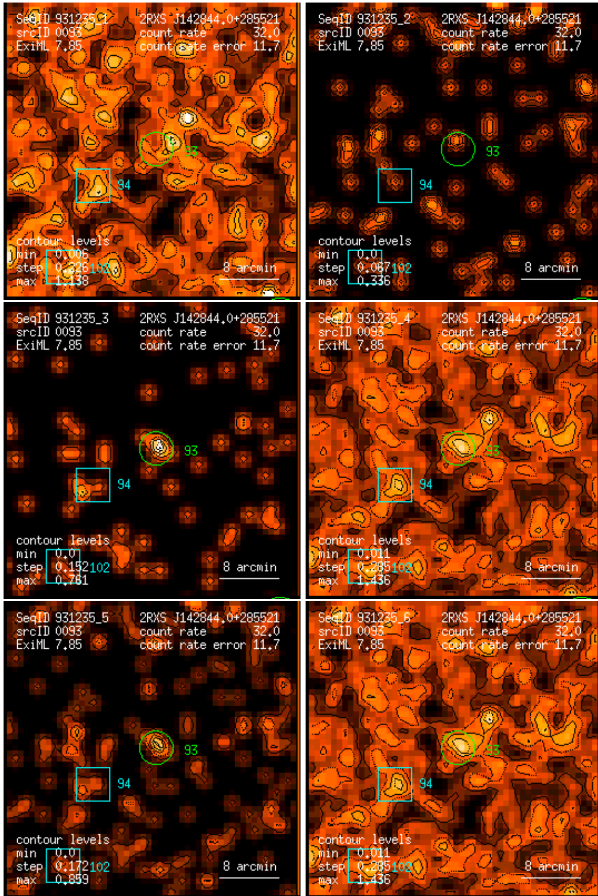
Figure 93: RASS 931235: detection 0093: band rate images, Gaussian filter: (1) PSPC channels 11 – 41, (2) 52 – 90, (3) 91 – 201, (4) 11 – 235, (5) 52 – 201, (6) 11 – 201. Broad band rates in counts/ks. Band rate contour levels in counts/ks/arcmin 2 .
