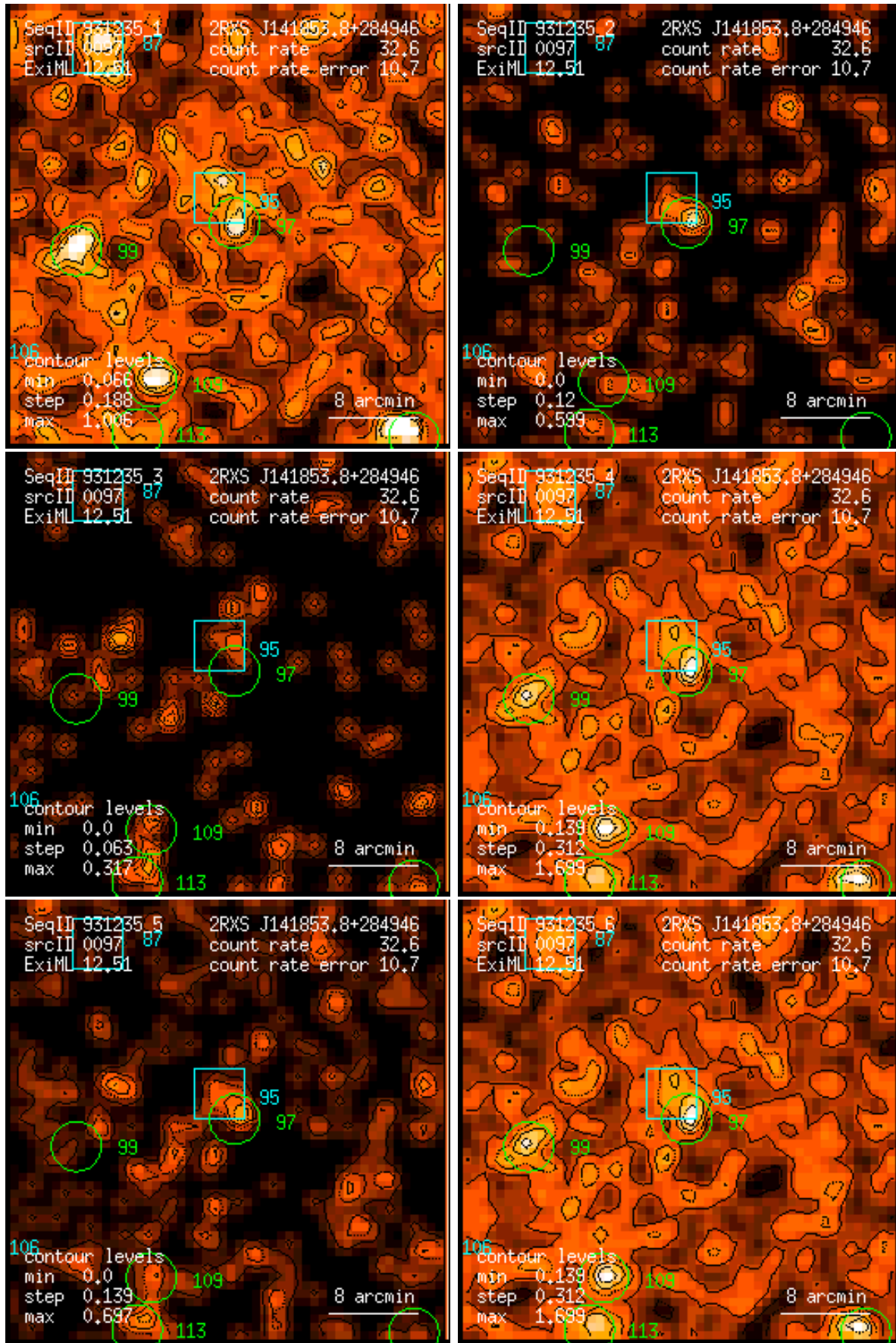
Figure 97: RASS 931235: detection 0097: band rate images, Gaussian filter: (1) PSPC channels 11 – 41, (2) 52 – 90, (3) 91 – 201, (4) 11 – 235, (5) 52 – 201, (6) 11 – 201. Broad band rates in counts/ks. Band rate contour levels in counts/ks/arcmin 2 .
