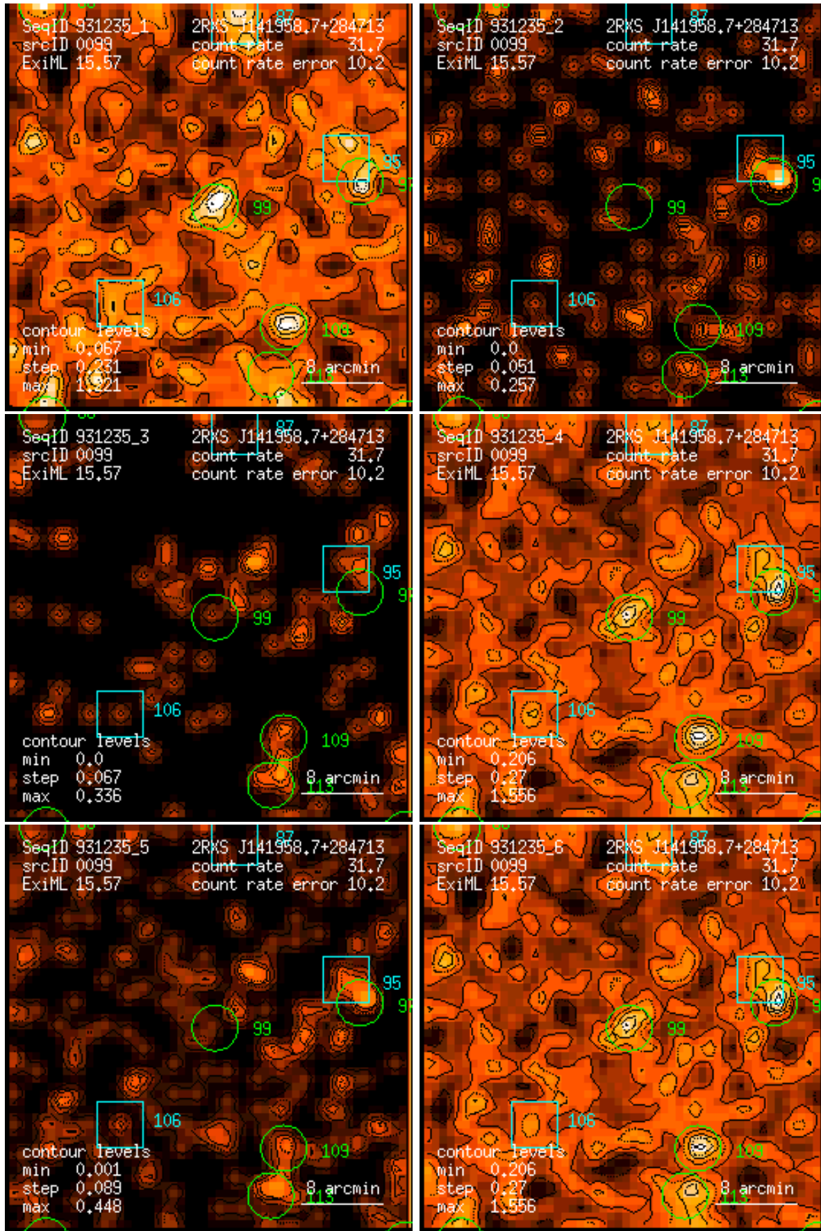
Figure 99: RASS 931235: detection 0099: band rate images, Gaussian filter: (1) PSPC channels 11 – 41, (2) 52 – 90, (3) 91 – 201, (4) 11 – 235, (5) 52 – 201, (6) 11 – 201. Broad band rates in counts/ks. Band rate contour levels in counts/ks/arcmin 2 .
