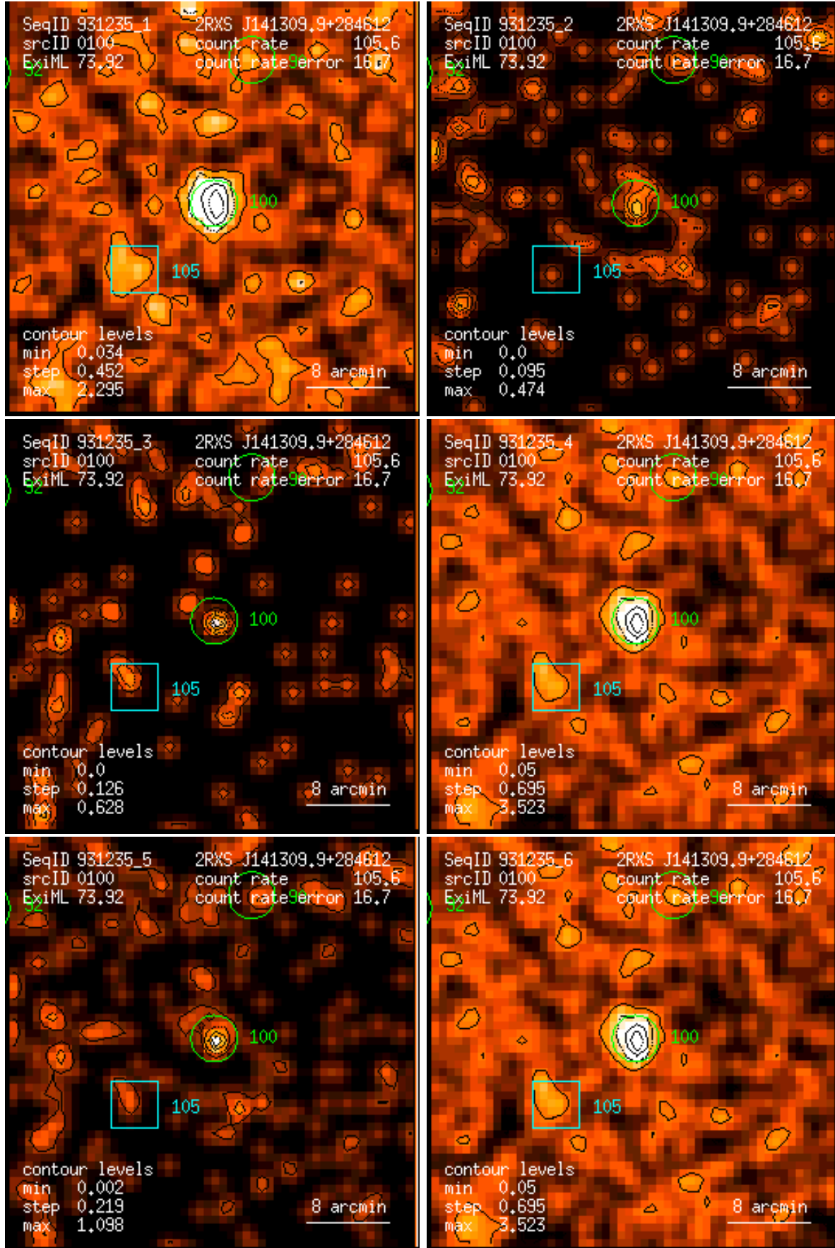
Figure 100: RASS 931235: detection 0100: band rate images, Gaussian filter: (1) PSPC channels 11 – 41, (2) 52 – 90, (3) 91 – 201, (4) 11 – 235, (5) 52 – 201, (6) 11 – 201. Broad band rates in counts/ks. Band rate contour levels in counts/ks/arcmin 2 .
