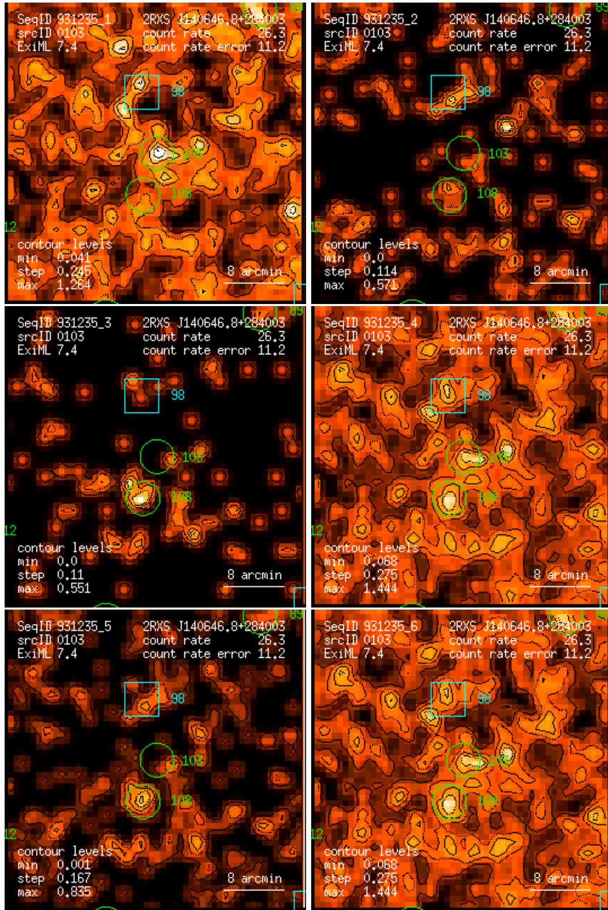
Figure 103: RASS 931235: detection 0103: band rate images, Gaussian filter: (1) PSPC channels 11 – 41, (2) 52 – 90, (3) 91 – 201, (4) 11 – 235, (5) 52 – 201, (6) 11 – 201. Broad band rates in counts/ks. Band rate contour levels in counts/ks/arcmin 2 .
