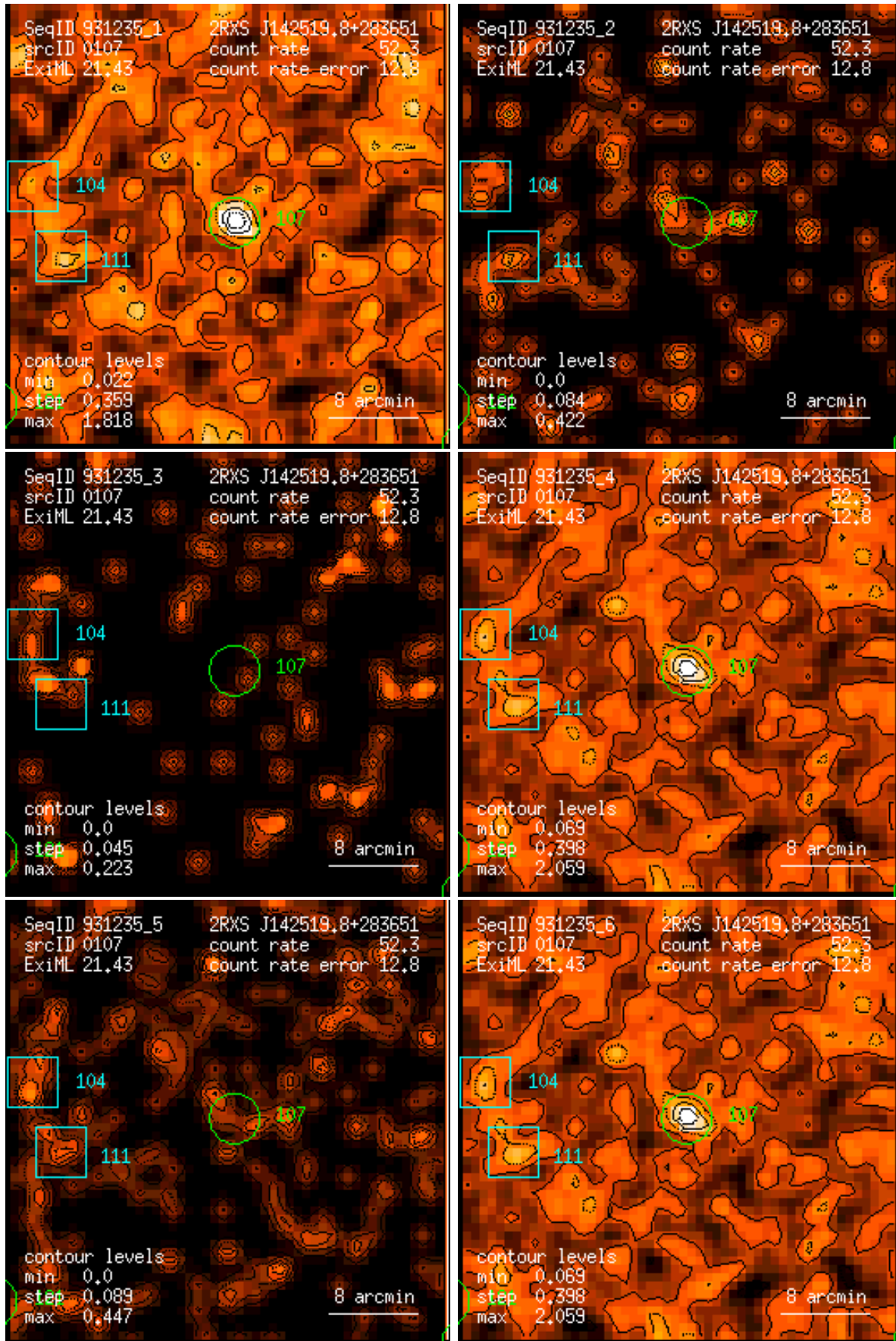
Figure 107: RASS 931235: detection 0107: band rate images, Gaussian filter: (1) PSPC channels 11 – 41, (2) 52 – 90, (3) 91 – 201, (4) 11 – 235, (5) 52 – 201, (6) 11 – 201. Broad band rates in counts/ks. Band rate contour levels in counts/ks/arcmin 2 .
