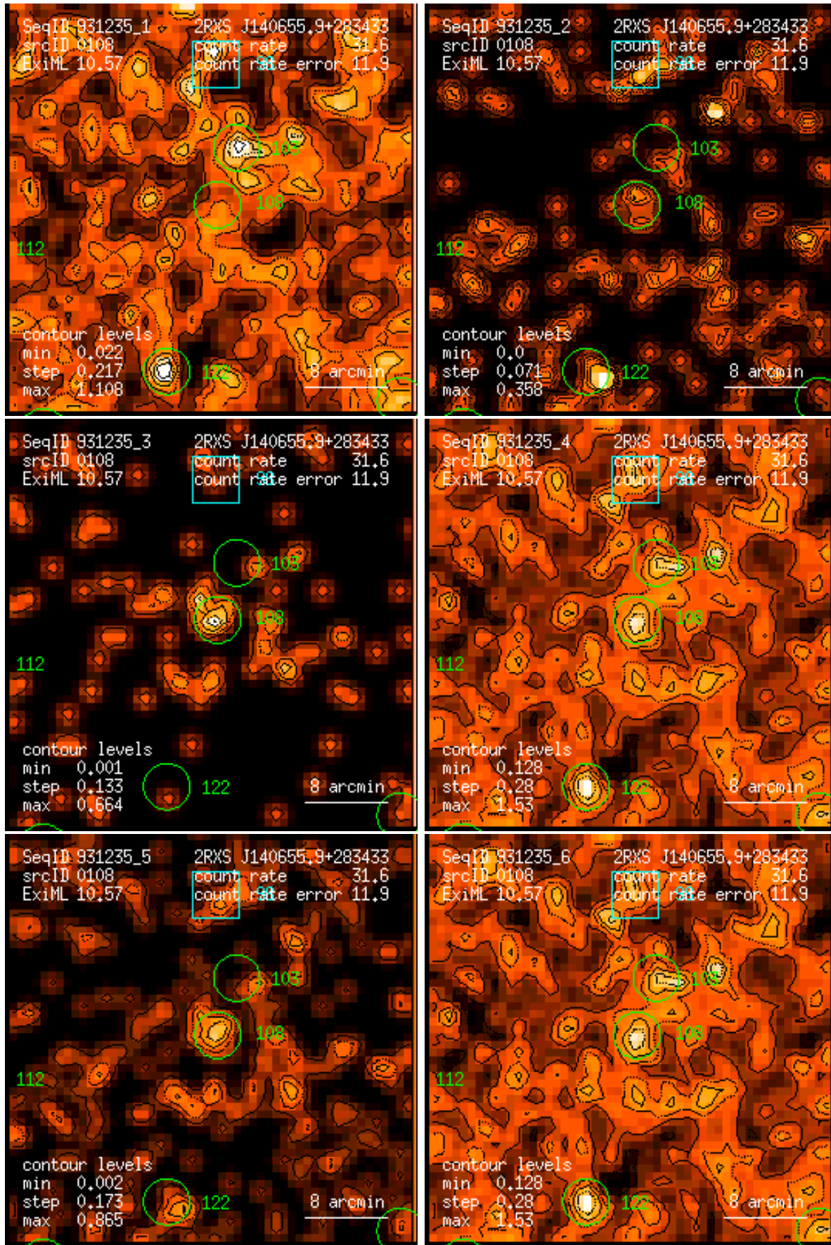
Figure 108: RASS 931235: detection 0108: band rate images, Gaussian filter: (1) PSPC channels 11 – 41, (2) 52 – 90, (3) 91 – 201, (4) 11 – 235, (5) 52 – 201, (6) 11 – 201. Broad band rates in counts/ks. Band rate contour levels in counts/ks/arcmin 2 .
