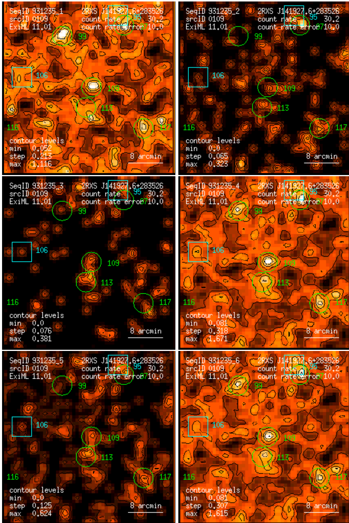
Figure 109: RASS 931235: detection 0109: band rate images, Gaussian filter: (1) PSPC channels 11 – 41, (2) 52 – 90, (3) 91 – 201, (4) 11 – 235, (5) 52 – 201, (6) 11 – 201. Broad band rates in counts/ks. Band rate contour levels in counts/ks/arcmin 2 .
