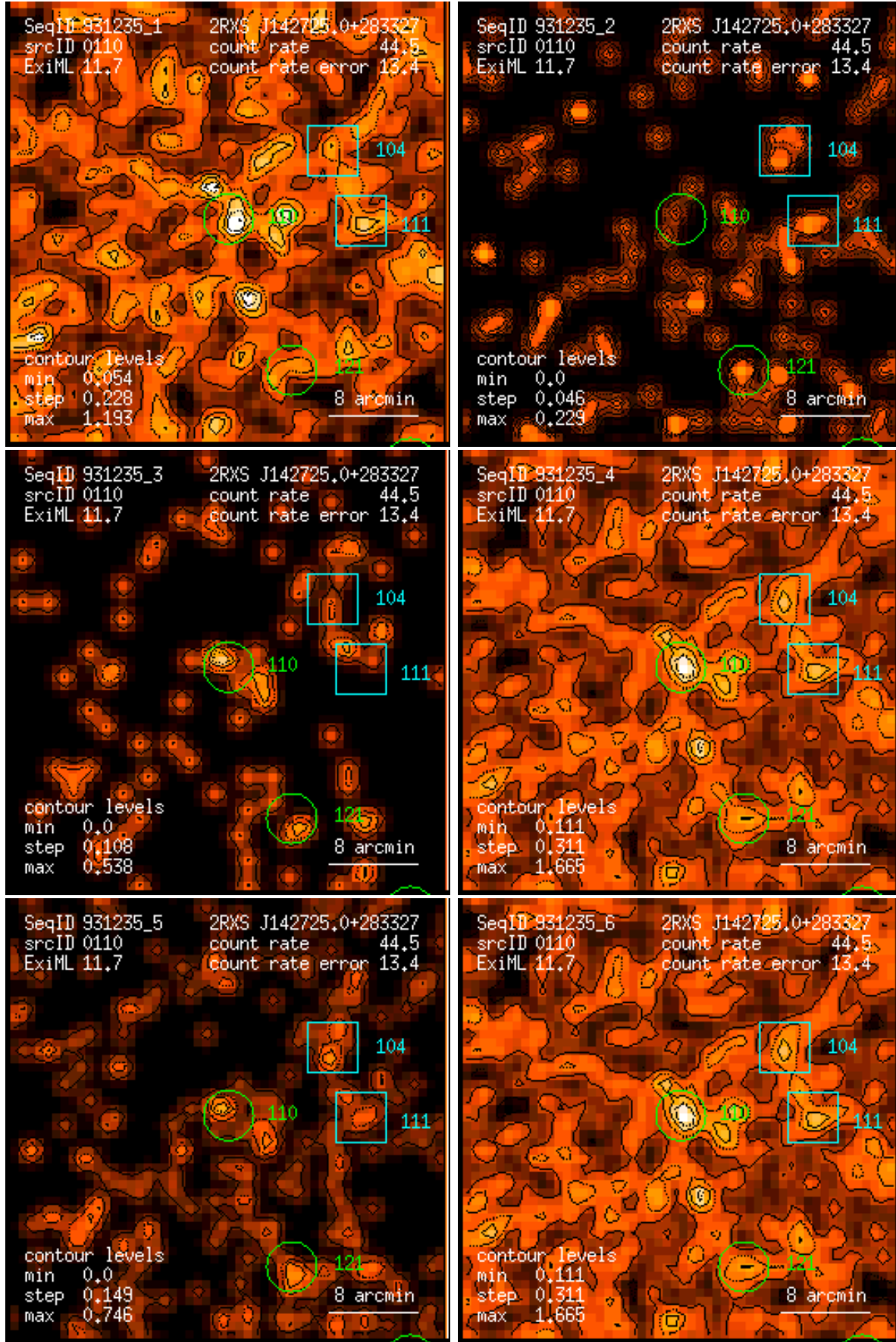
Figure 110: RASS 931235: detection 0110: band rate images, Gaussian filter: (1) PSPC channels 11 – 41, (2) 52 – 90, (3) 91 – 201, (4) 11 – 235, (5) 52 – 201, (6) 11 – 201. Broad band rates in counts/ks. Band rate contour levels in counts/ks/arcmin 2 .
