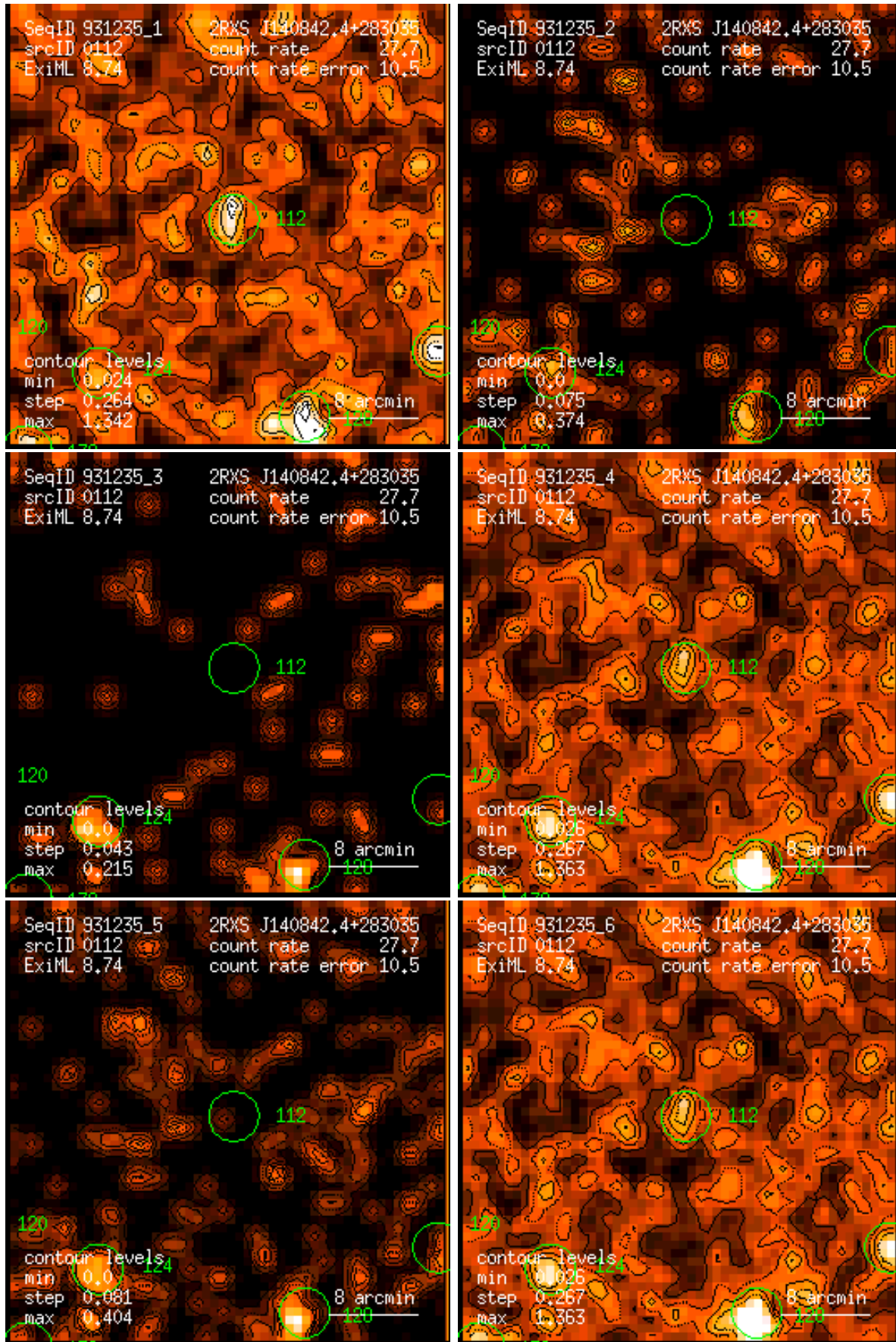
Figure 112: RASS 931235: detection 0112: band rate images, Gaussian filter: (1) PSPC channels 11 – 41, (2) 52 – 90, (3) 91 – 201, (4) 11 – 235, (5) 52 – 201, (6) 11 – 201. Broad band rates in counts/ks. Band rate contour levels in counts/ks/arcmin 2 .
