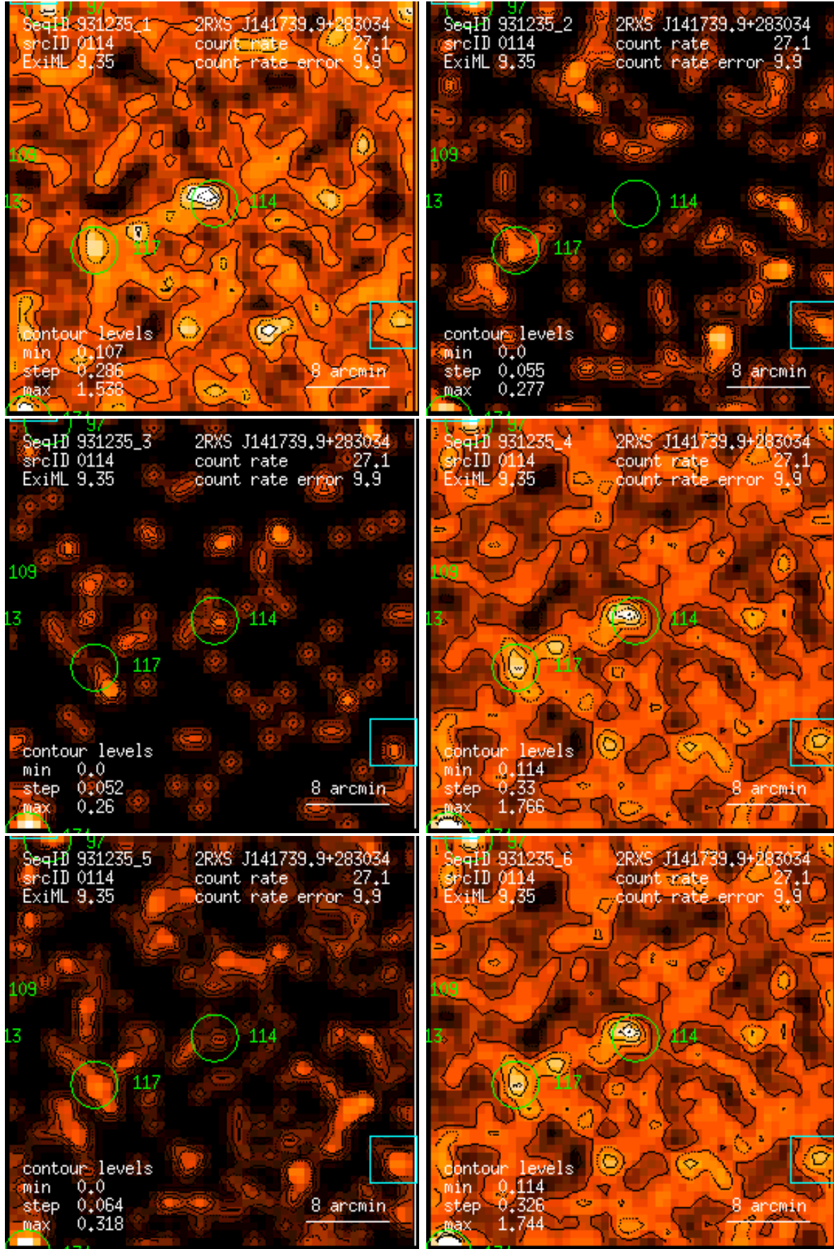
Figure 114: RASS 931235: detection 0114: band rate images, Gaussian filter: (1) PSPC channels 11 – 41, (2) 52 – 90, (3) 91 – 201, (4) 11 – 235, (5) 52 – 201, (6) 11 – 201. Broad band rates in counts/ks. Band rate contour levels in counts/ks/arcmin 2 .
