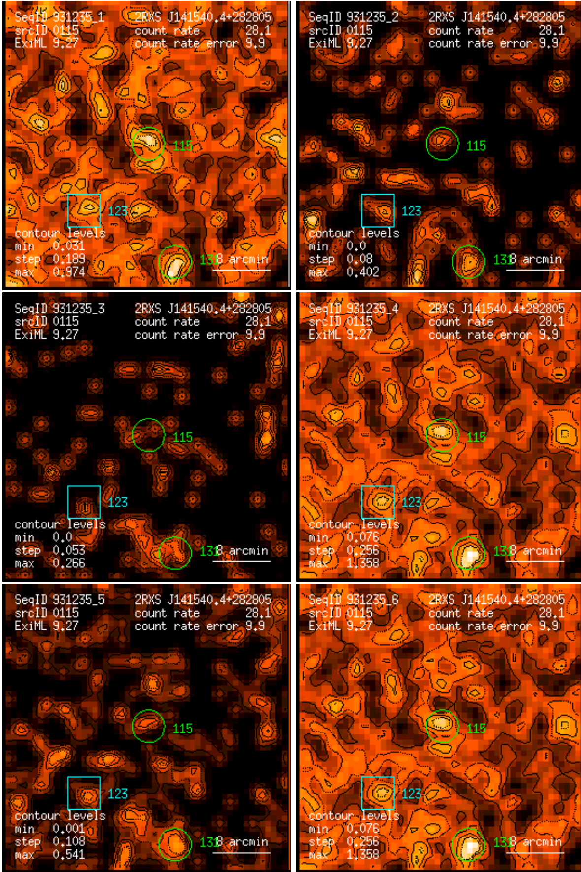
Figure 115: RASS 931235: detection 0115: band rate images, Gaussian filter: (1) PSPC channels 11 – 41, (2) 52 – 90, (3) 91 – 201, (4) 11 – 235, (5) 52 – 201, (6) 11 – 201. Broad band rates in counts/ks. Band rate contour levels in counts/ks/arcmin 2 .
