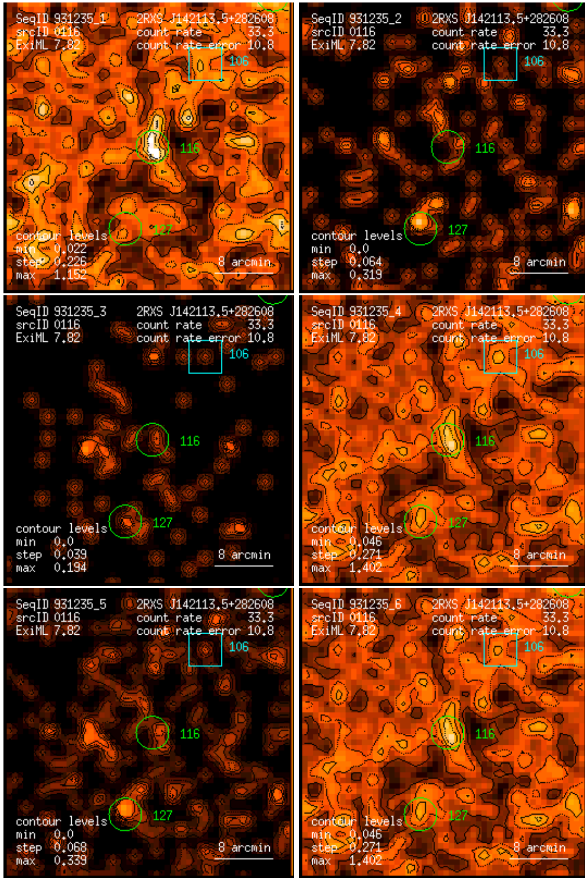
Figure 116: RASS 931235: detection 0116: band rate images, Gaussian filter: (1) PSPC channels 11 – 41, (2) 52 – 90, (3) 91 – 201, (4) 11 – 235, (5) 52 – 201, (6) 11 – 201. Broad band rates in counts/ks. Band rate contour levels in counts/ks/arcmin 2 .
