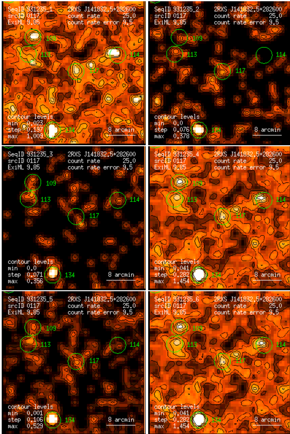
Figure 117: RASS 931235: detection 0117: band rate images, Gaussian filter: (1) PSPC channels 11 – 41, (2) 52 – 90, (3) 91 – 201, (4) 11 – 235, (5) 52 – 201, (6) 11 – 201. Broad band rates in counts/ks. Band rate contour levels in counts/ks/arcmin 2 .
