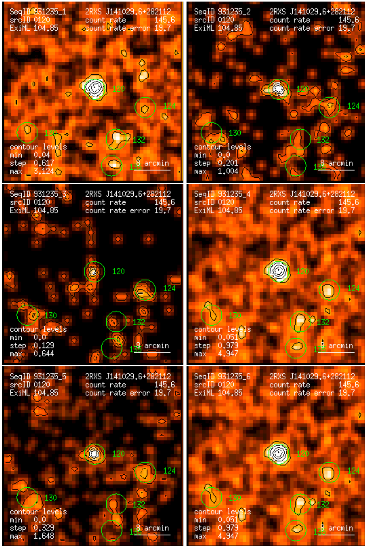
Figure 120: RASS 931235: detection 0120: band rate images, Gaussian filter: (1) PSPC channels 11 – 41, (2) 52 – 90, (3) 91 – 201, (4) 11 – 235, (5) 52 – 201, (6) 11 – 201. Broad band rates in counts/ks. Band rate contour levels in counts/ks/arcmin 2 .
