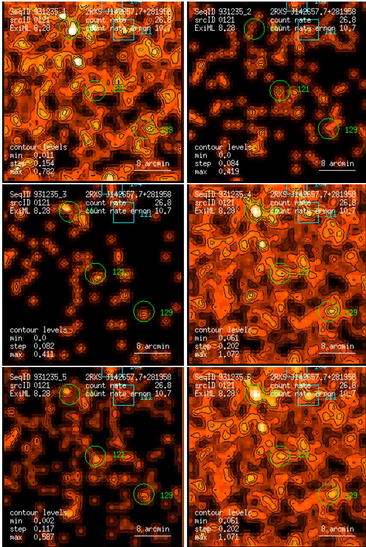
Figure 121: RASS 931235: detection 0121: band rate images, Gaussian filter: (1) PSPC channels 11 – 41, (2) 52 – 90, (3) 91 – 201, (4) 11 – 235, (5) 52 – 201, (6) 11 – 201. Broad band rates in counts/ks. Band rate contour levels in counts/ks/arcmin 2 .
