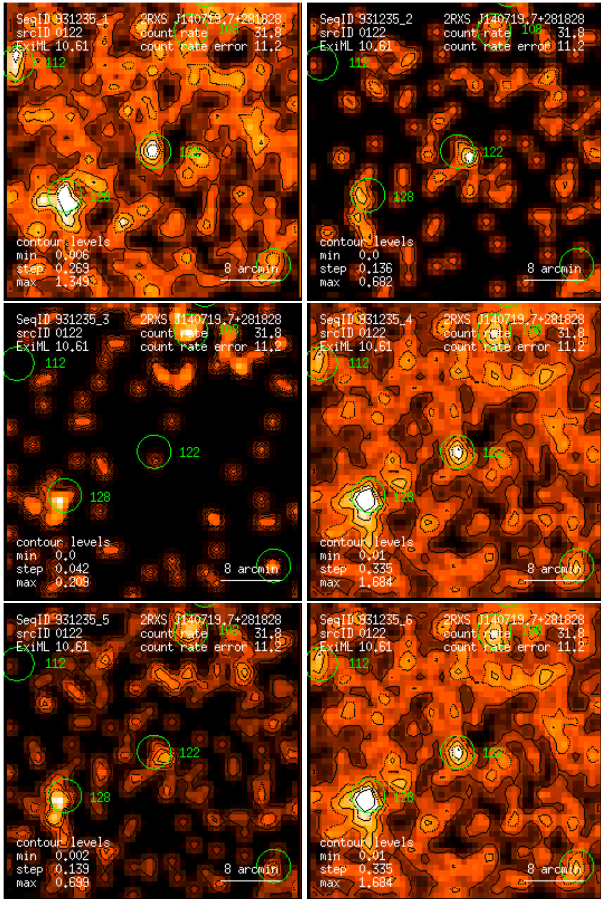
Figure 122: RASS 931235: detection 0122: band rate images, Gaussian filter: (1) PSPC channels 11 – 41, (2) 52 – 90, (3) 91 – 201, (4) 11 – 235, (5) 52 – 201, (6) 11 – 201. Broad band rates in counts/ks. Band rate contour levels in counts/ks/arcmin 2 .
