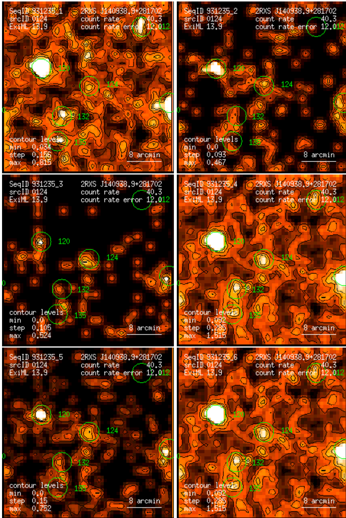
Figure 124: RASS 931235: detection 0124: band rate images, Gaussian filter: (1) PSPC channels 11 – 41, (2) 52 – 90, (3) 91 – 201, (4) 11 – 235, (5) 52 – 201, (6) 11 – 201. Broad band rates in counts/ks. Band rate contour levels in counts/ks/arcmin 2 .
