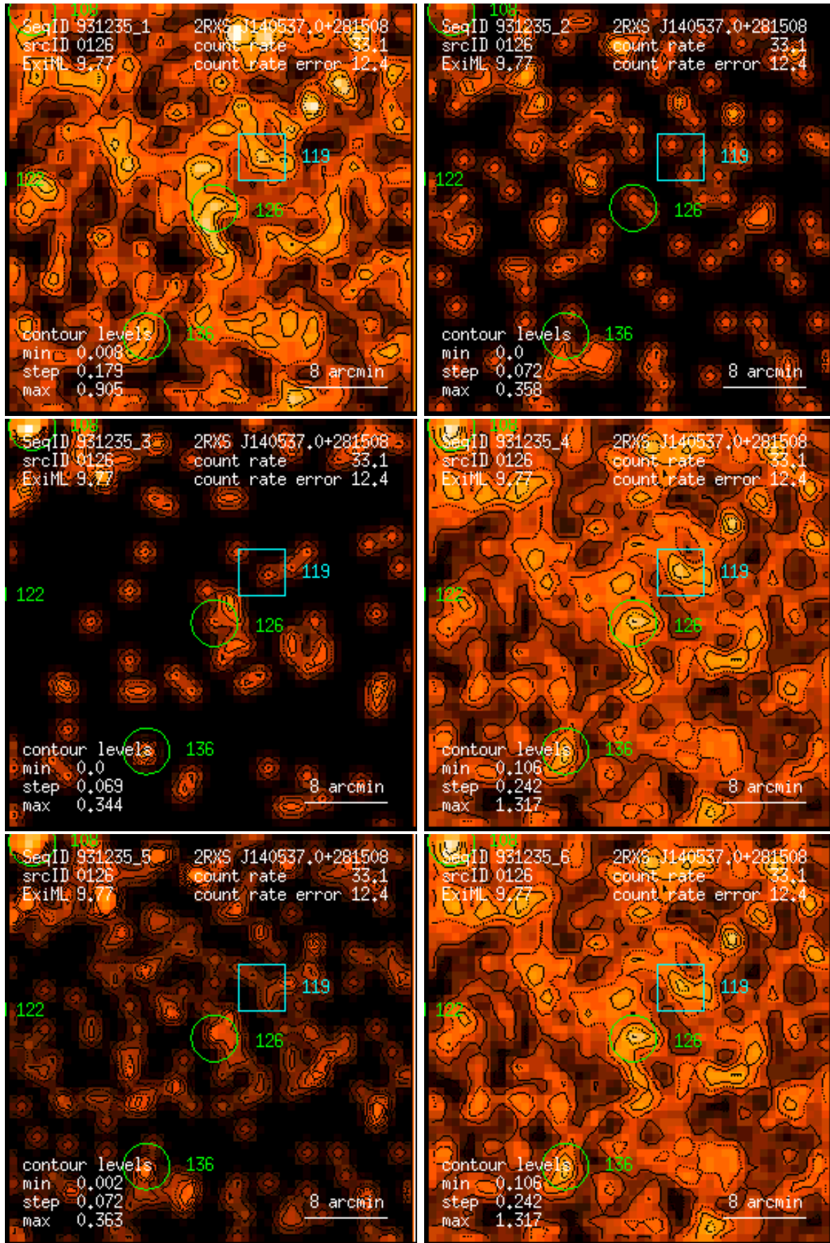
Figure 126: RASS 931235: detection 0126: band rate images, Gaussian filter: (1) PSPC channels 11 – 41, (2) 52 – 90, (3) 91 – 201, (4) 11 – 235, (5) 52 – 201, (6) 11 – 201. Broad band rates in counts/ks. Band rate contour levels in counts/ks/arcmin 2 .
