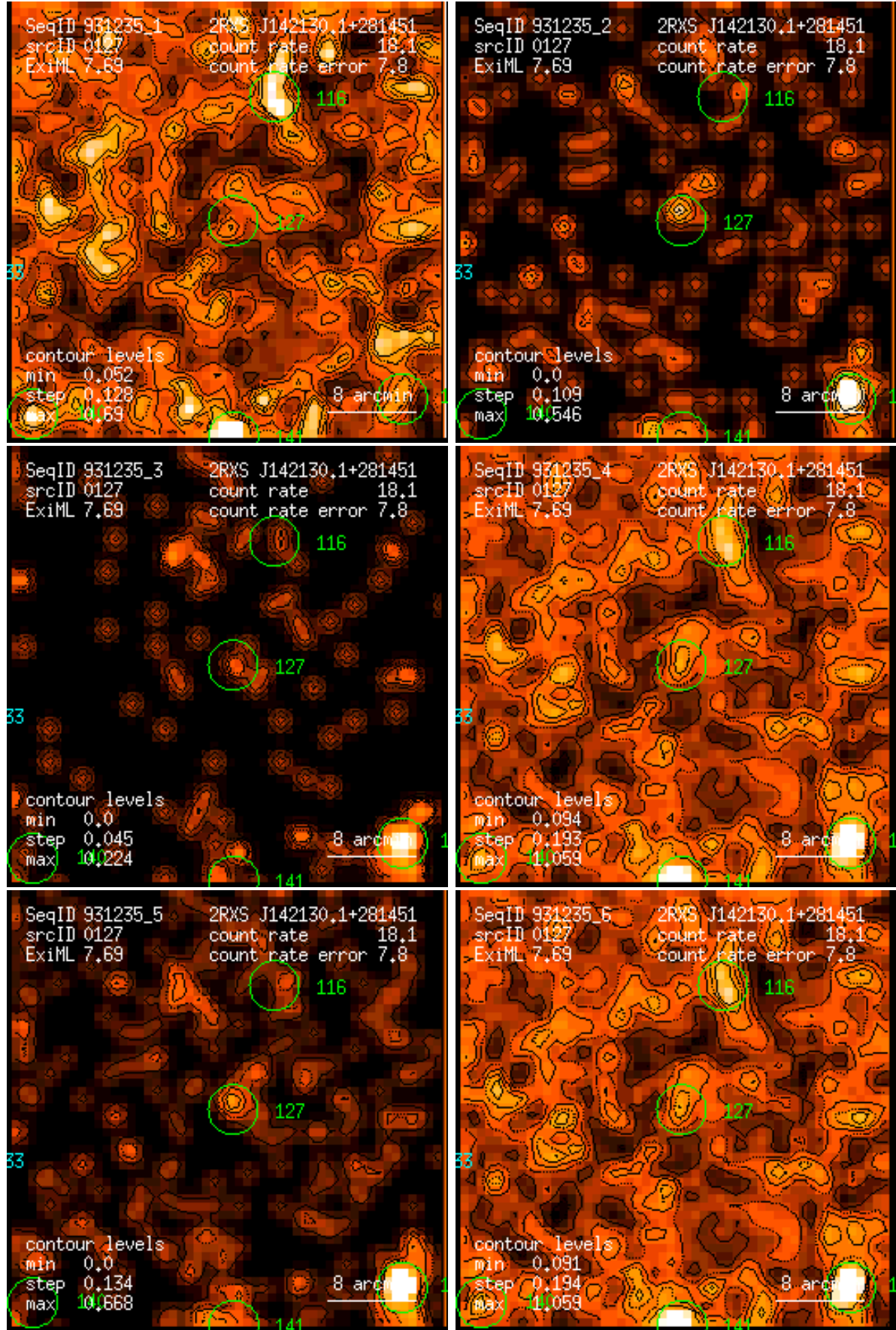
Figure 127: RASS 931235: detection 0127: band rate images, Gaussian filter: (1) PSPC channels 11 – 41, (2) 52 – 90, (3) 91 – 201, (4) 11 – 235, (5) 52 – 201, (6) 11 – 201. Broad band rates in counts/ks. Band rate contour levels in counts/ks/arcmin 2 .
